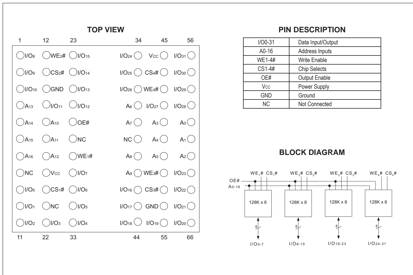
FIGURE 1 – PIN CONFIGURATION FOR WE128K32N-XH1X
