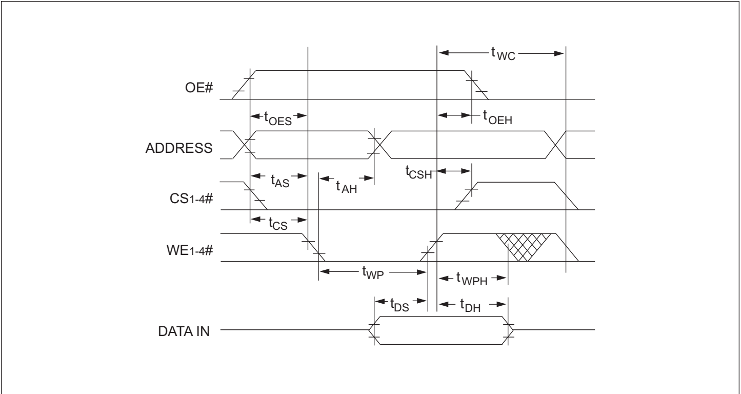
FIGURE 5 – WRITE WAVEFORMS WE# CONTROLLED
