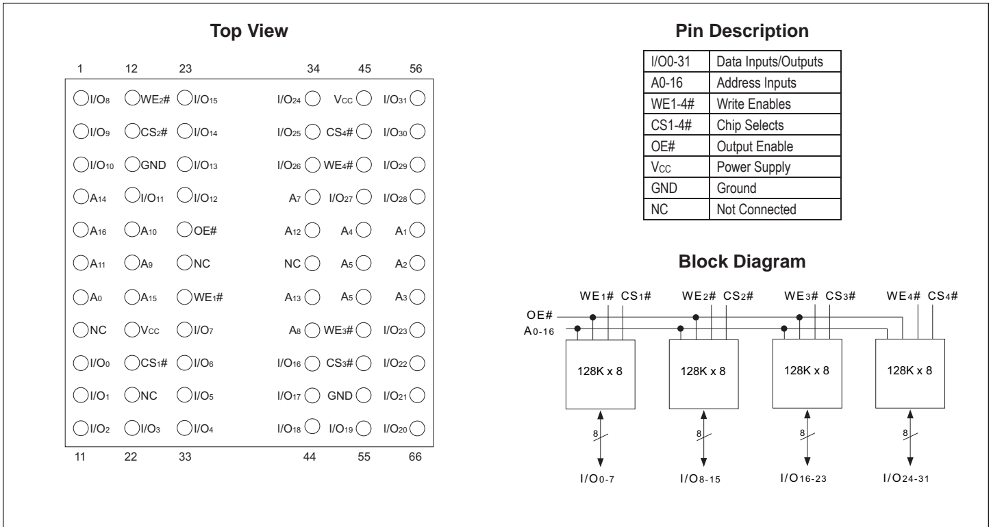
FIGURE 12 – ALTERNATE PIN CONFIGURATION FOR WE128K32NP-XH1X
