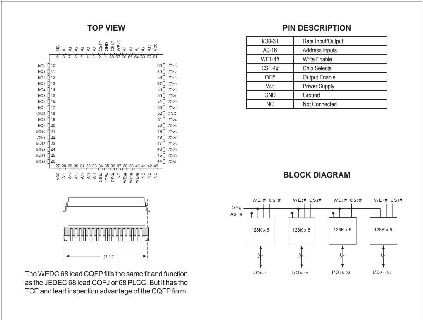
FIGURE 3 – PIN CONFIGURATION FOR WE128K32-XG2TX
