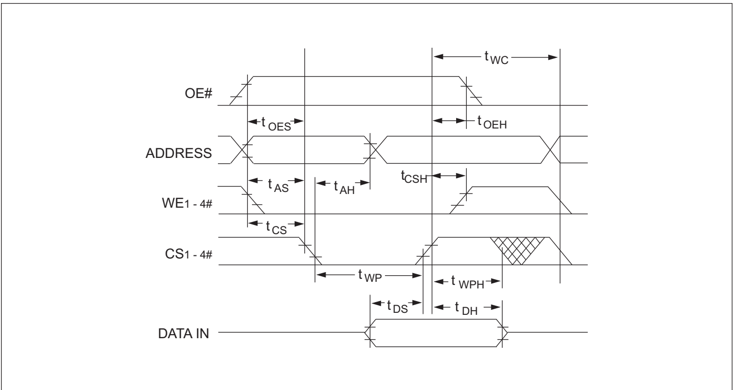
FIGURE 6 – WRITE WAVEFORMS CS# CONTROLLED
