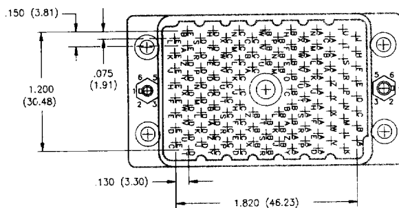
120 PIN PLUG
