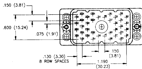
38 PIN PLUG
