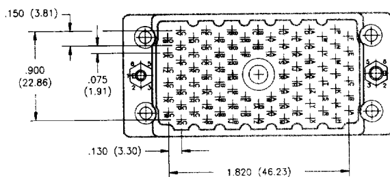
90 PIN PLUG
