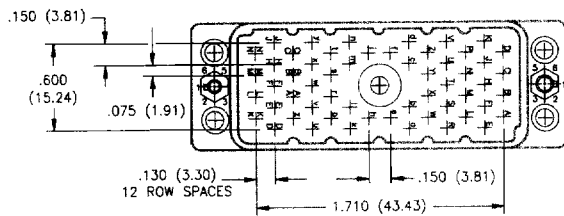
56 PIN PLUG
