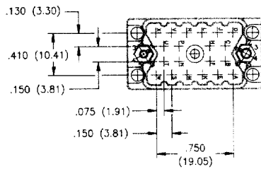
20 PIN PLUG
