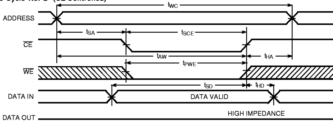
Write Cycle No. 2 ( \overline{CE} Controlled) [11.14]
