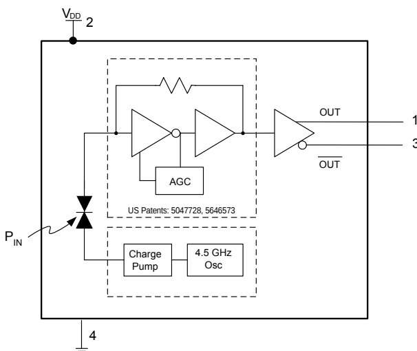
Figure 1: Equivalent Circuit
