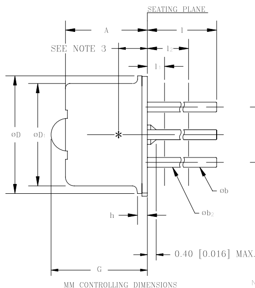
MM CONTROLLING DIMENSIONS
