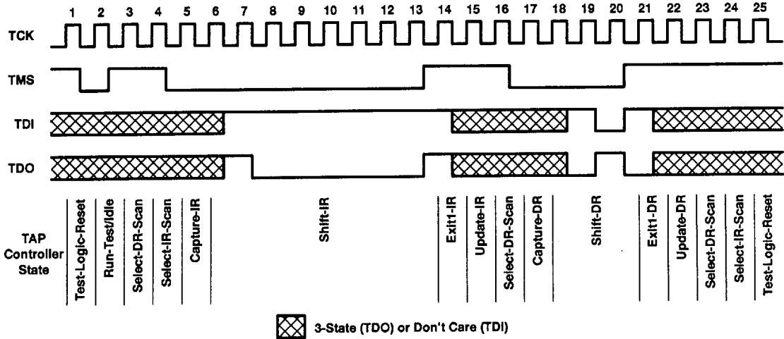
Figure 14. Timing Example
