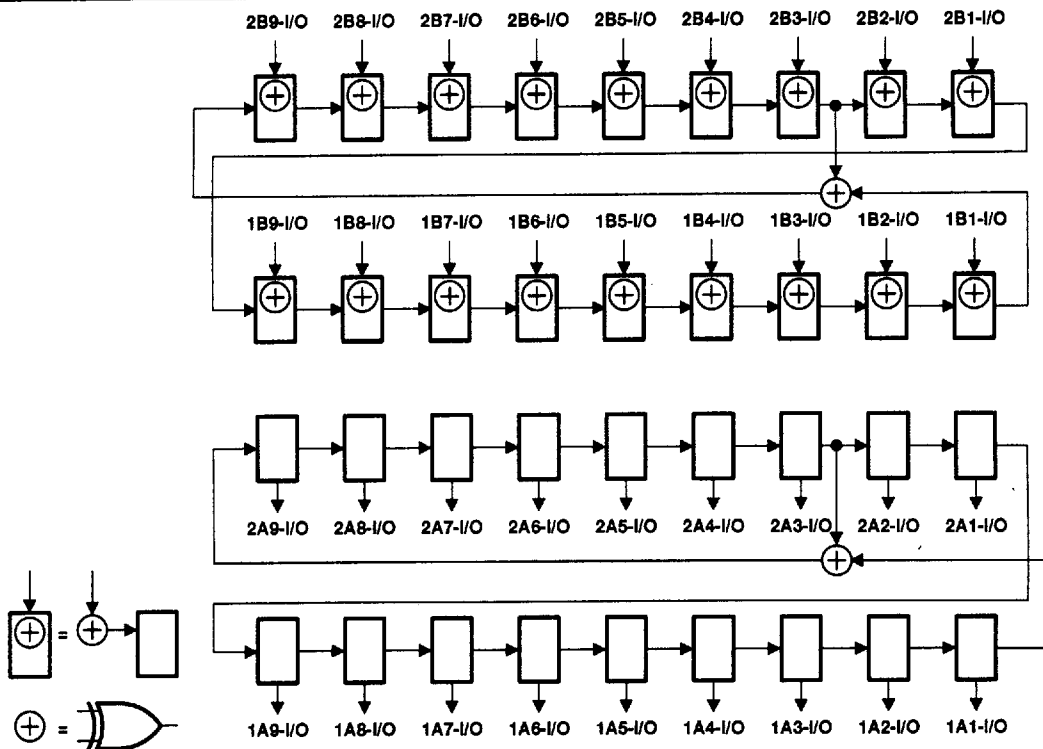
Figure 11. 18-Bit PSA/PRPG Configuration (10EA = 20EA = 1, 10EB = 20EB = 0)
