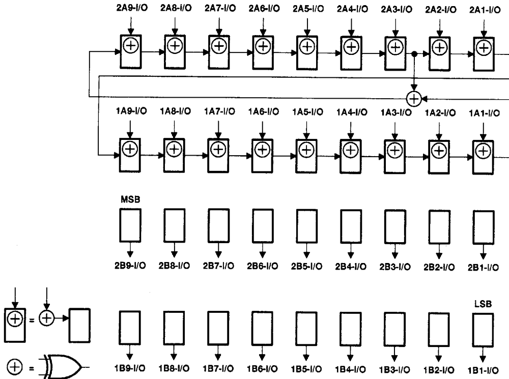
Figure 12. 18-Bit PSA/COUNT Configuration (10EA = 20EA = 0, 10EB = 20EB = 1)
