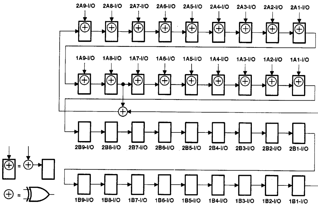
Figure 8. 36-Bit PSA Configuration (10EA = 20EA = 0, 10EB = 20EB = 1)
