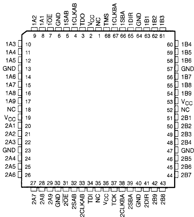
SN54LVT18646, SN54LVT182646... HV PACKAGE (TOP VIEW)
