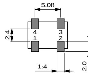
PC board footprint
