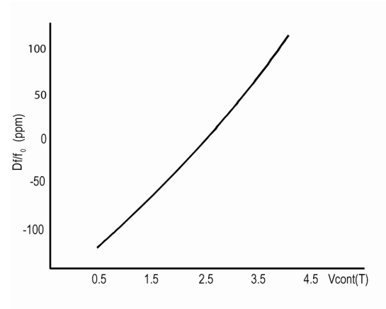
Typical Voltage Control Curve @ 25°C & 20.0MHz
