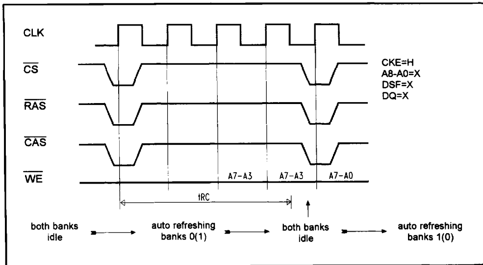
Figure 22. Timing and control for Auto Refresh Operation
