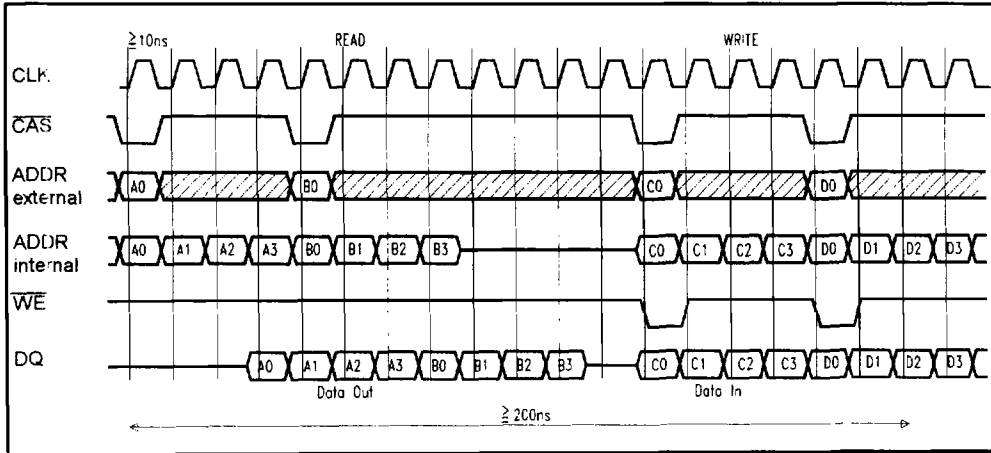
Figure 28. Timing of pipeline operation, latency = 3, burst length = 4
