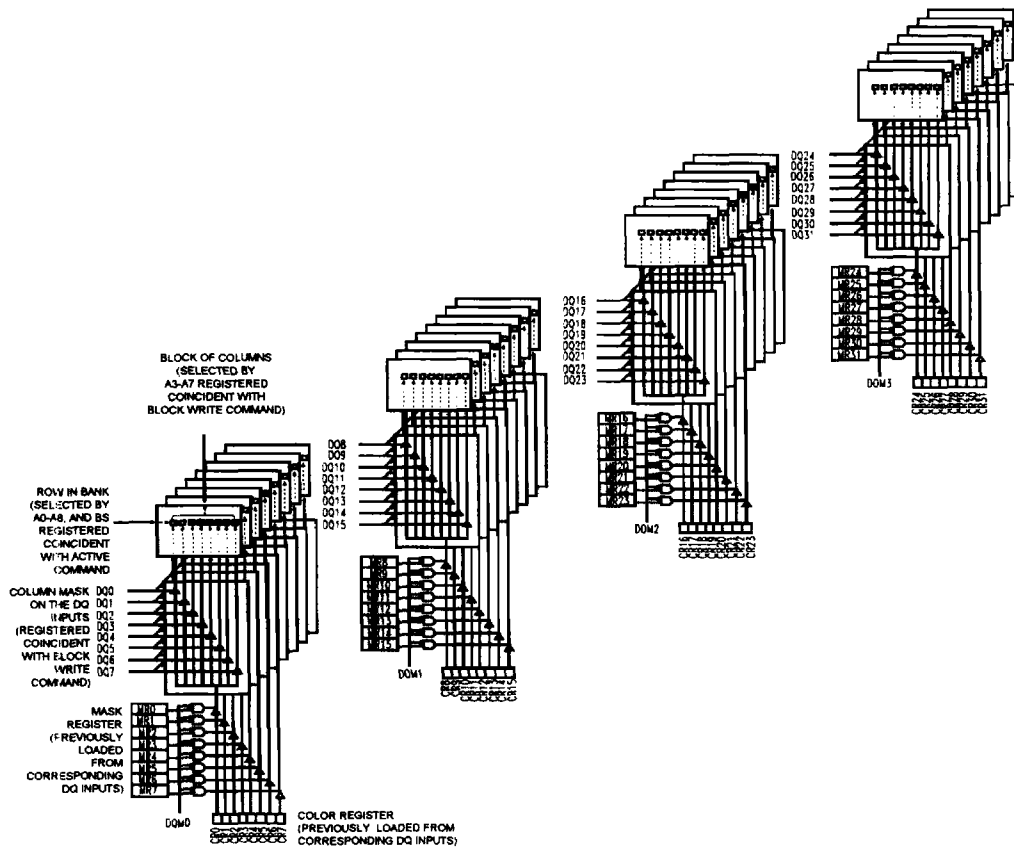
Figure 19. Diagram of block write operation
