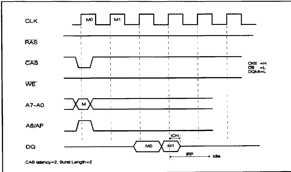
Figure 15. Read burst with Auto Precharge selected
