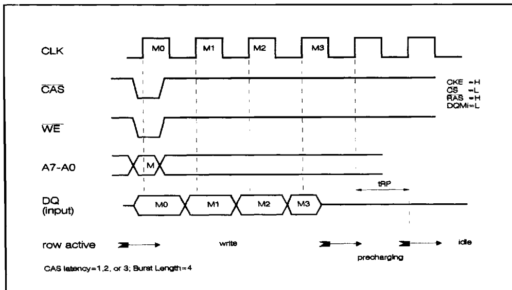
Figure 17. Write burst Auto Precharge selected
