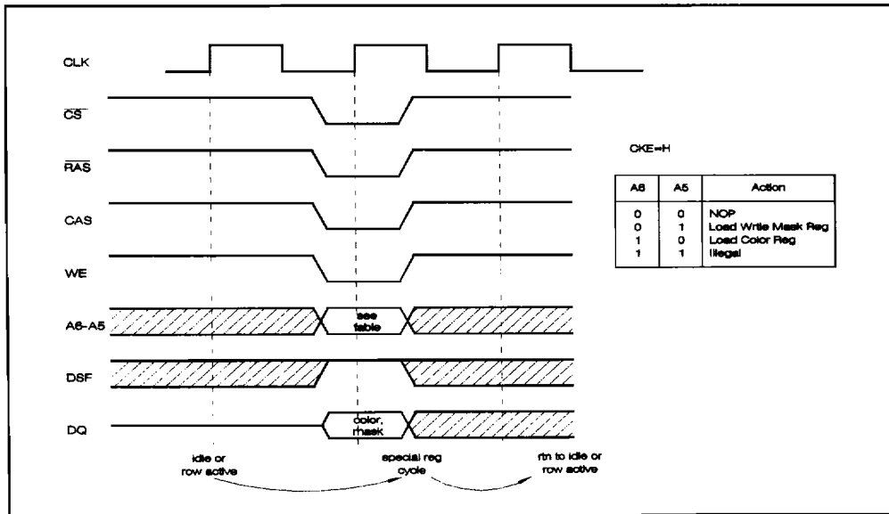
Figure 7. Timing and control for special register access cycle
