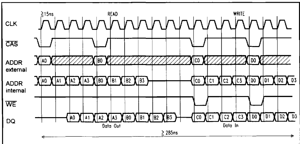
Figure 27. Timing of pipeline operation, latency = 2, burst length = 4
