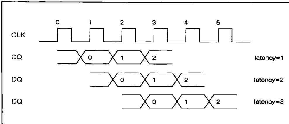
Figure 5. Definition of Read Latency with Examples
