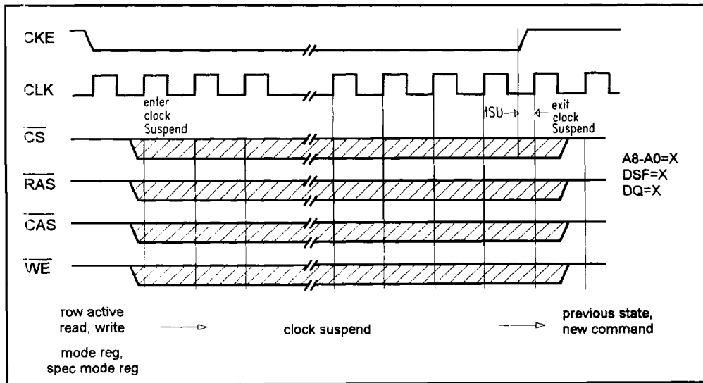
Figure 25. Example timing and control for Clock suspend operation
