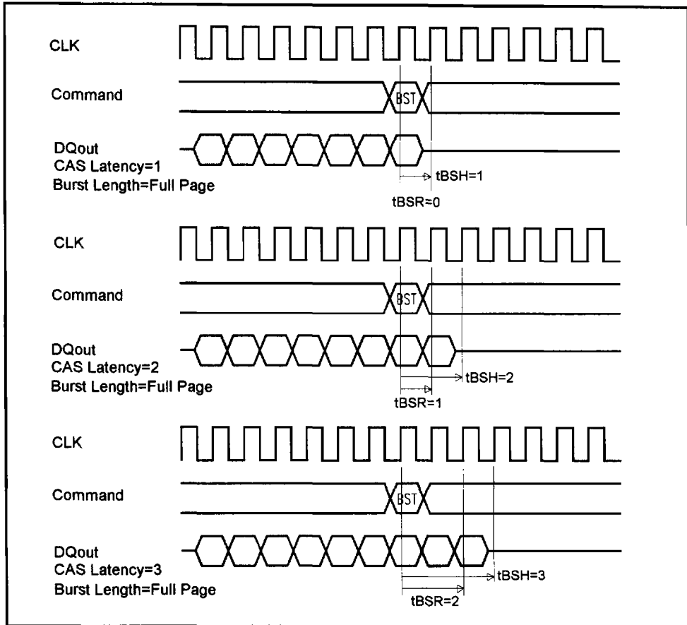
Figure 13-1. Full page burst stop
