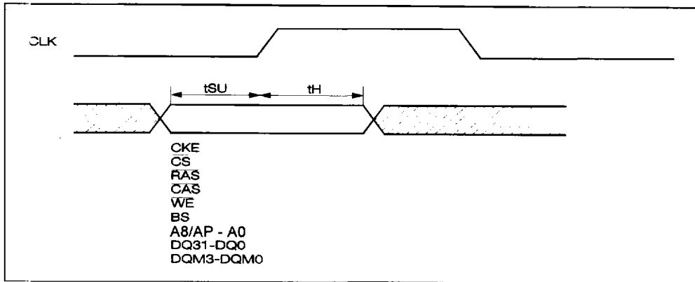
Figure 3. General Cycle Invocation Scheme for SGRAM
