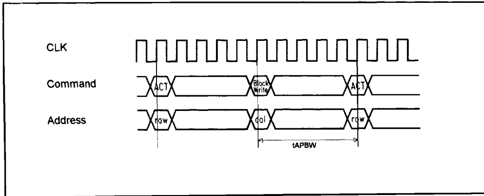
Figure 21. Timing of Block Write with auto precharge selected
