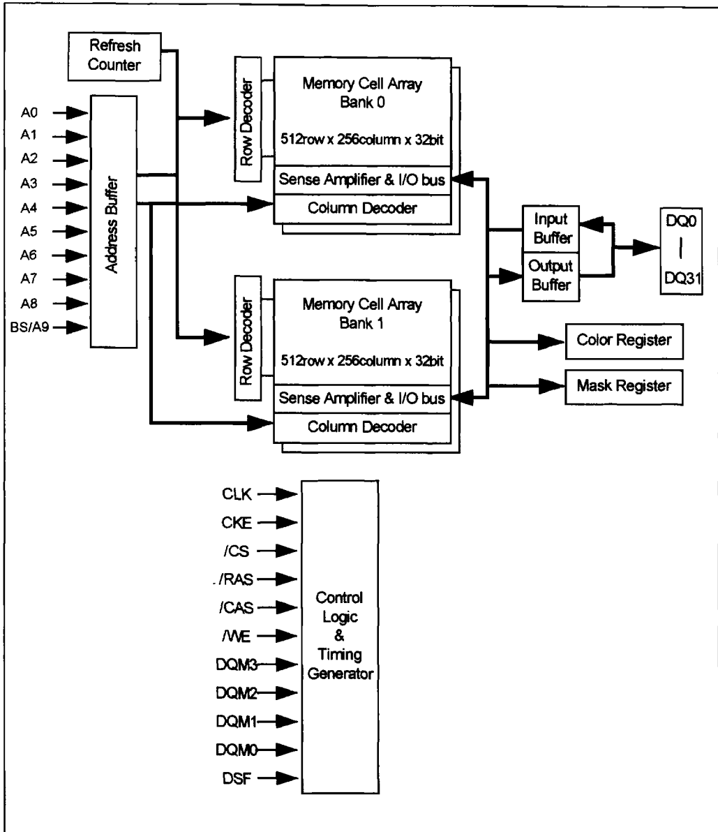
Figure 2. Simplified Block Diagram
