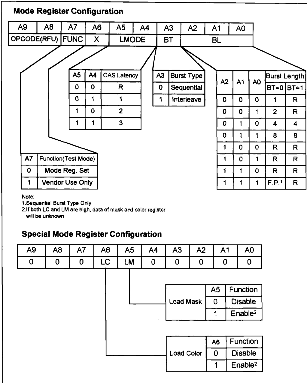
Figure 8. Loading of the mode register and special mode register
