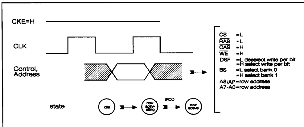
Figure 9. Row activate command to idle bank
