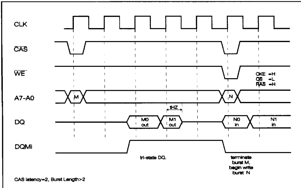
Figure 12. Timing of write initiation with read burst in progress
