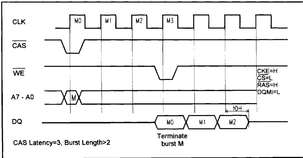
Figure 13. Timing of burst terminate command with read burst in progress
