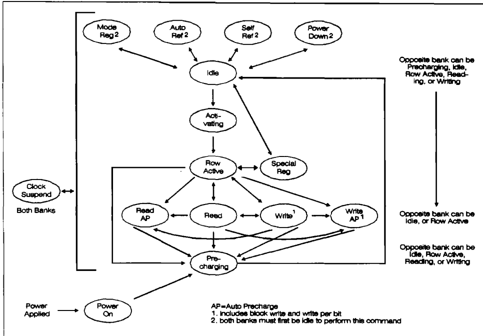
Figure 4. Simplified state transition diagram for each bank.
