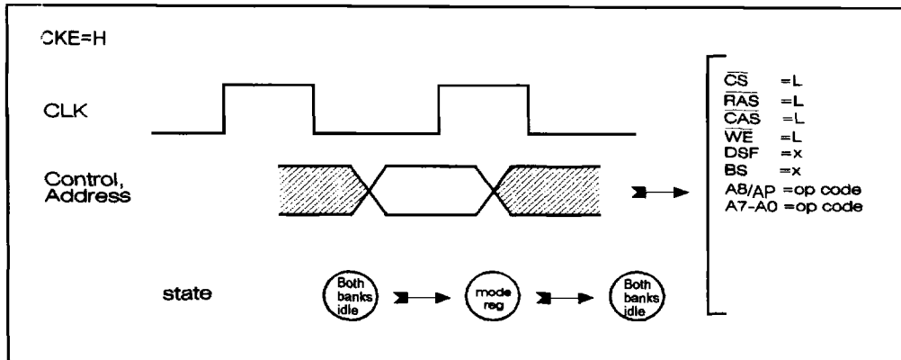
Figure 6. Timing of mode register access (Program latency and burst length)
