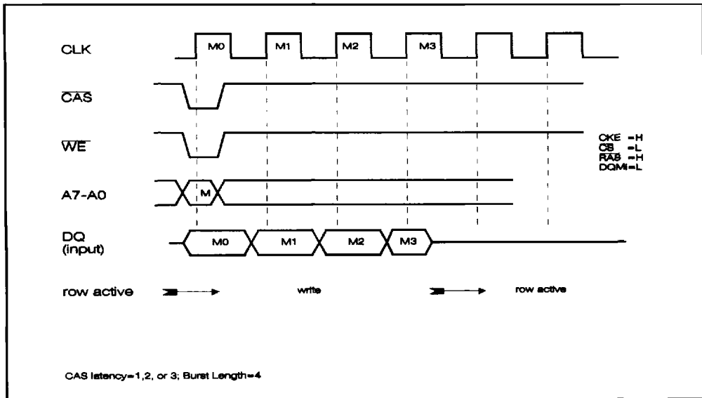
Figure 16. Write burst with Auto Precharge deselected.
