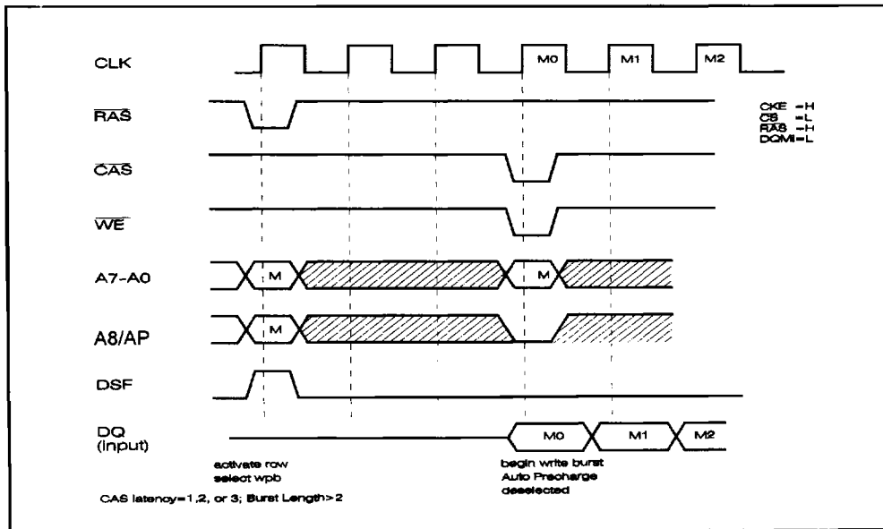
Figure 18. Write burst with Write Per Bit, Auto Precharge deselected
