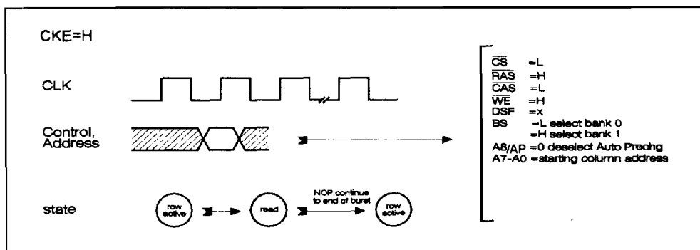
Figure 10. Burst read sequence, Auto Precharge Deselected
