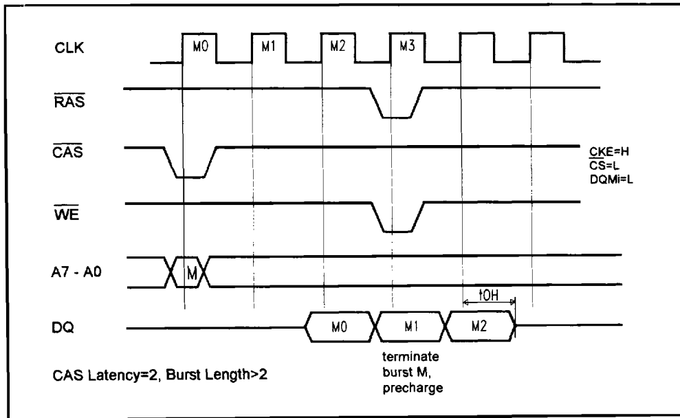
Figure 14. Timing of precharge command with read burst in progress
