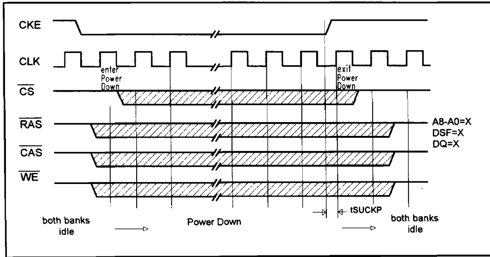
Figure 24. Example timing and control for Power down operation
