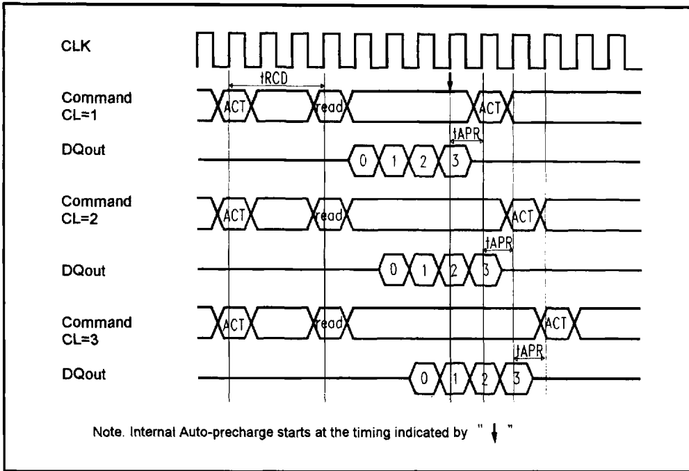
Figure 15-1. Burst read with auto precharge followed by an active command
