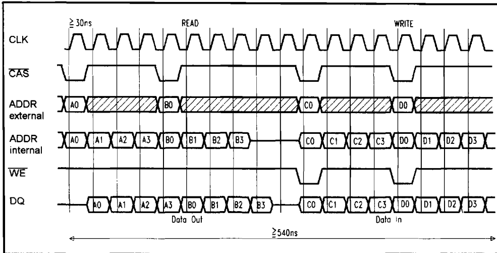
Figure 26. Timing of pipeline operation, latency = 1, burst length = 4
