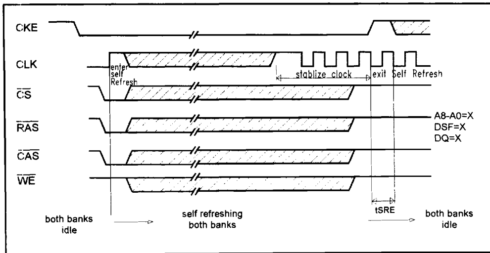
Figure 23. Timing and control for Self Refresh Operation
