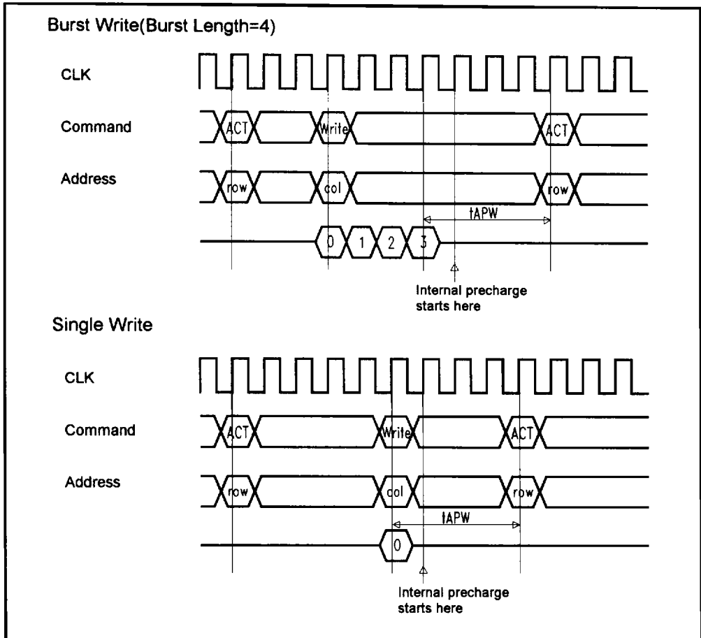
Figure 17-1. Write burst with Auto Precharge followed by an active command
