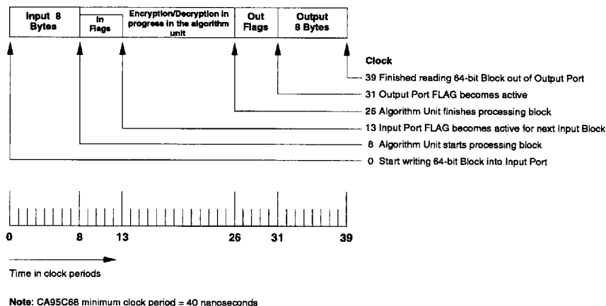
Figure 3-22 : Detailed Timing of One Block
