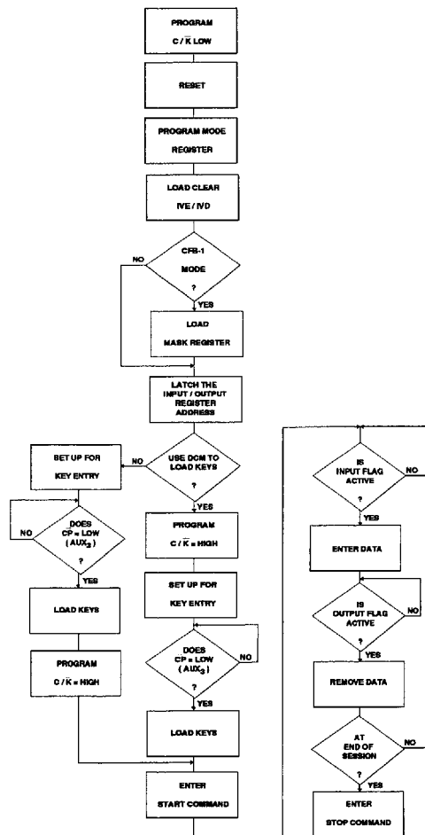
Figure 3-21 : Direct Control Mode CBC/CFB Programming Flow Chart
