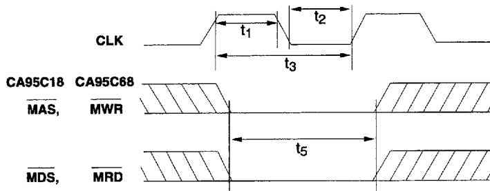
Figure 3-8 : CA95C68/18 Clock and Reset Timing
