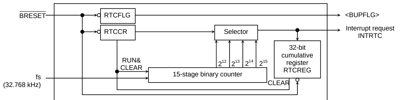
Fig. 17.6.1 Block Diagram of the Clock Timer
