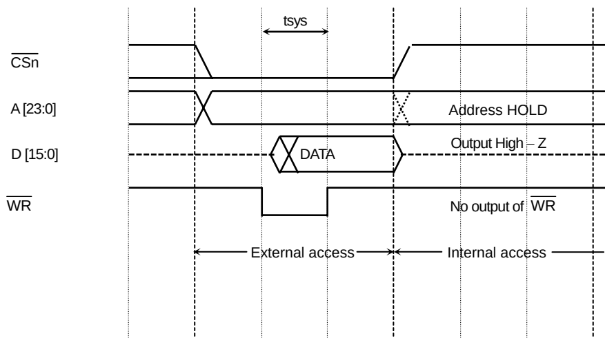
Fig. 8.3.2 Write Operation Timing Diagram
