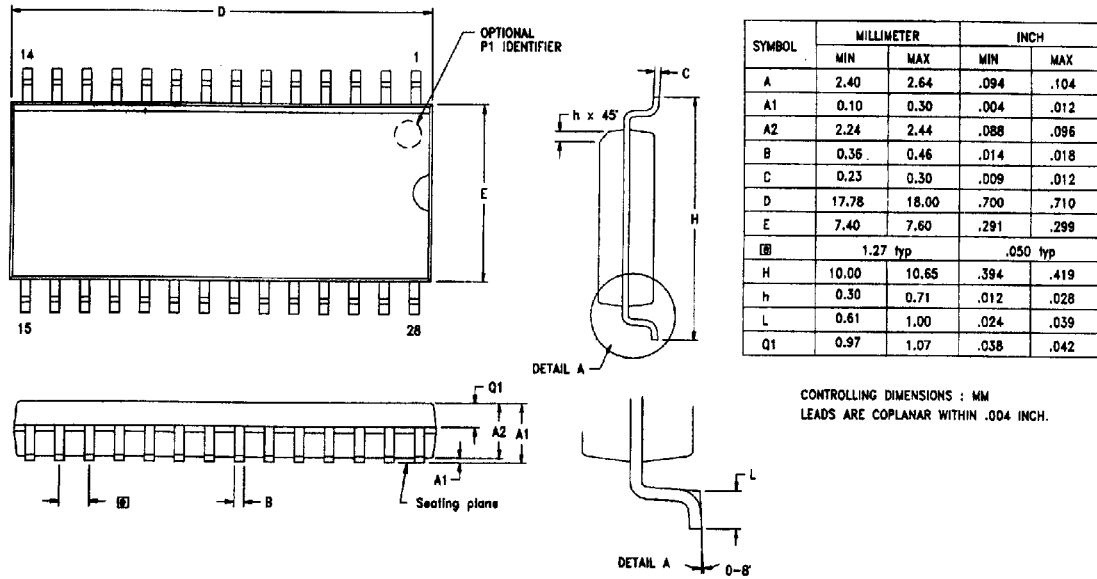
Figure 6. 28-pin SOIC Package Diagram
