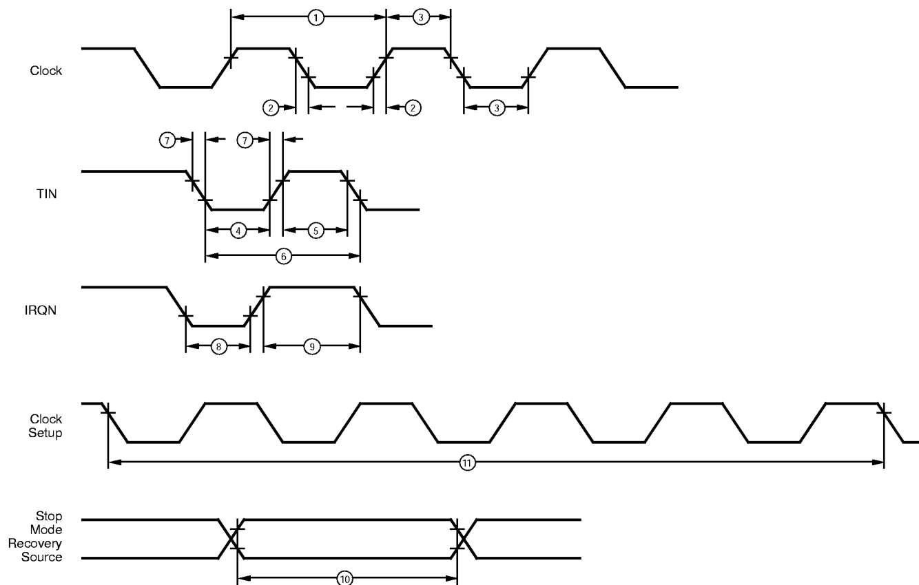
Figure 3. Additional Timing
