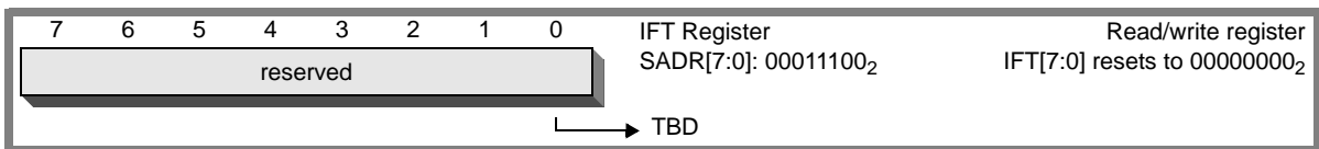
Figure 41 : DA Register
