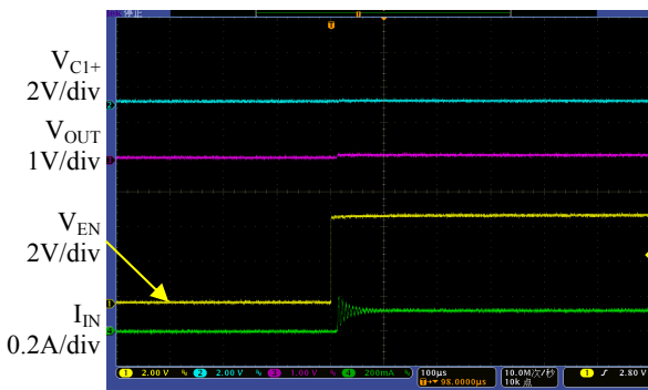
Time (100µs/div)
