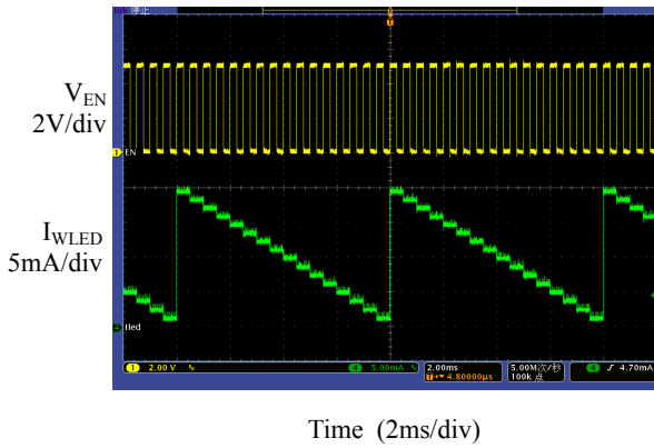
Figure 28. 1x Mode Dimming Operation (AP3606, V_{IN}=5\text{V} , f_{EN}=2\text{kHz} )
