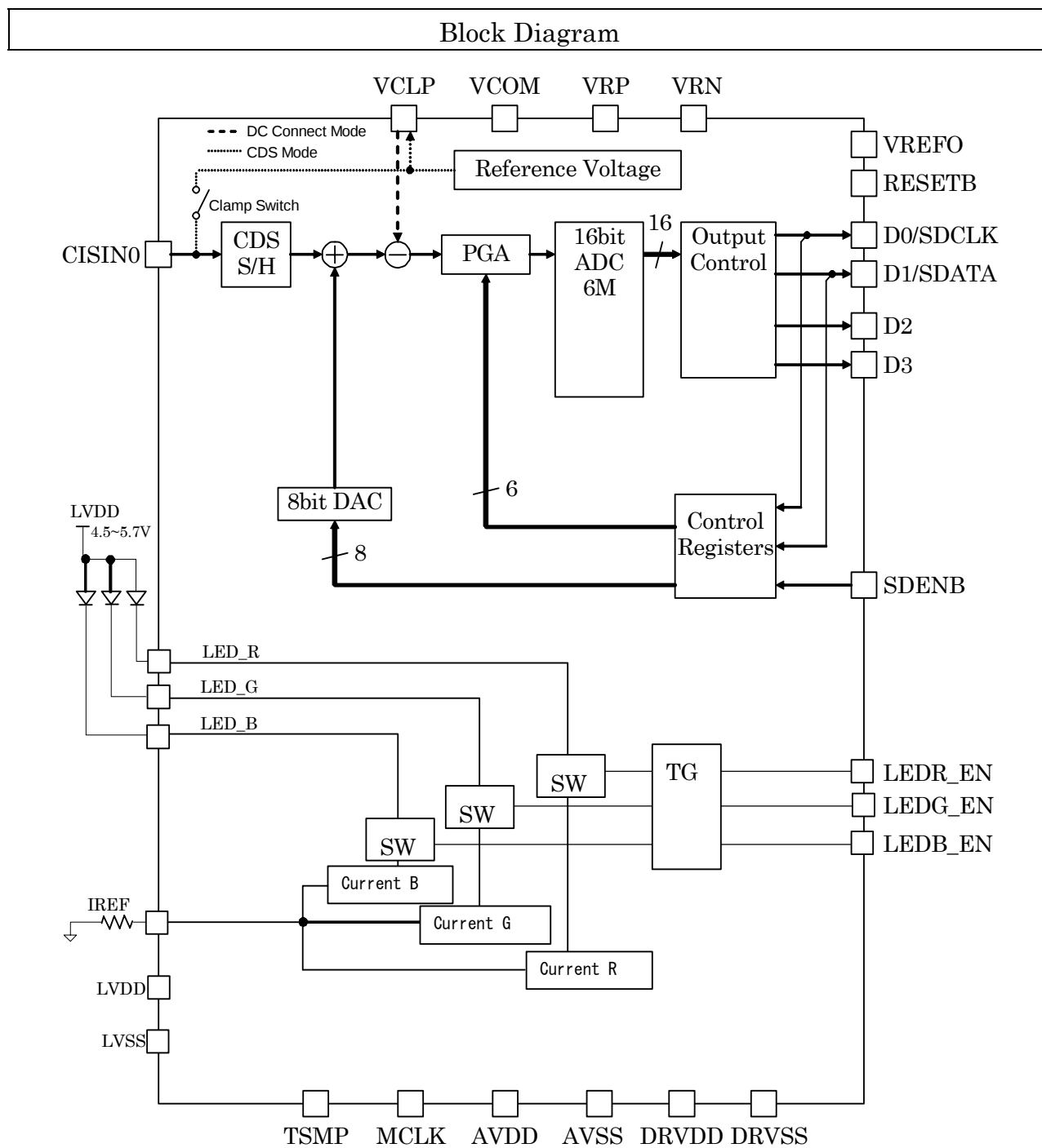
Fig. 1 Block diagram
