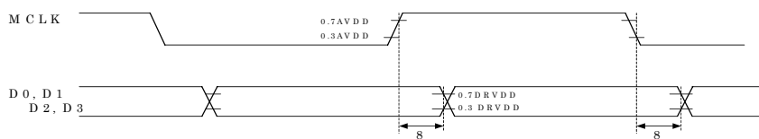
Data output timing ( Double edge mode )
