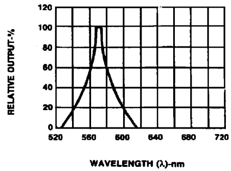
Fig.2 SPECTRAL RESPONSE
