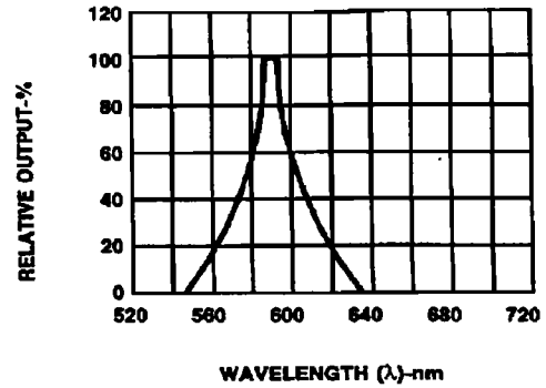
Fig.2 SPECTRAL RESPONSE
