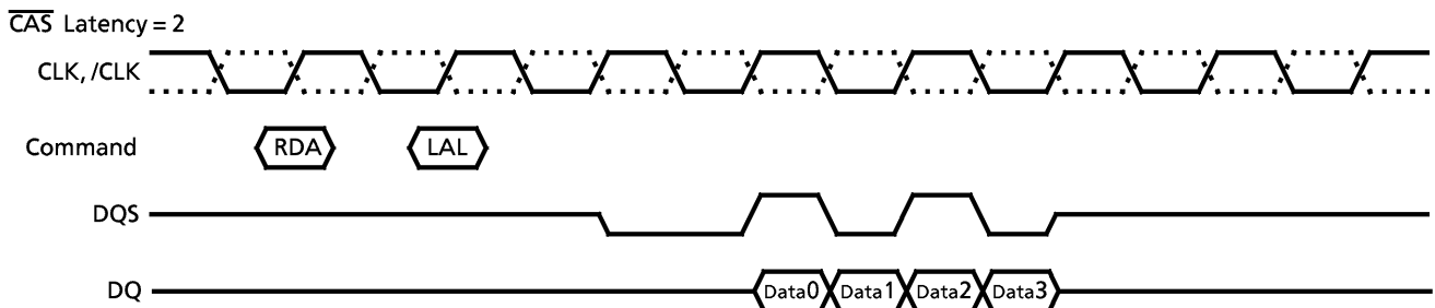
Addressing sequence for Sequential mode
