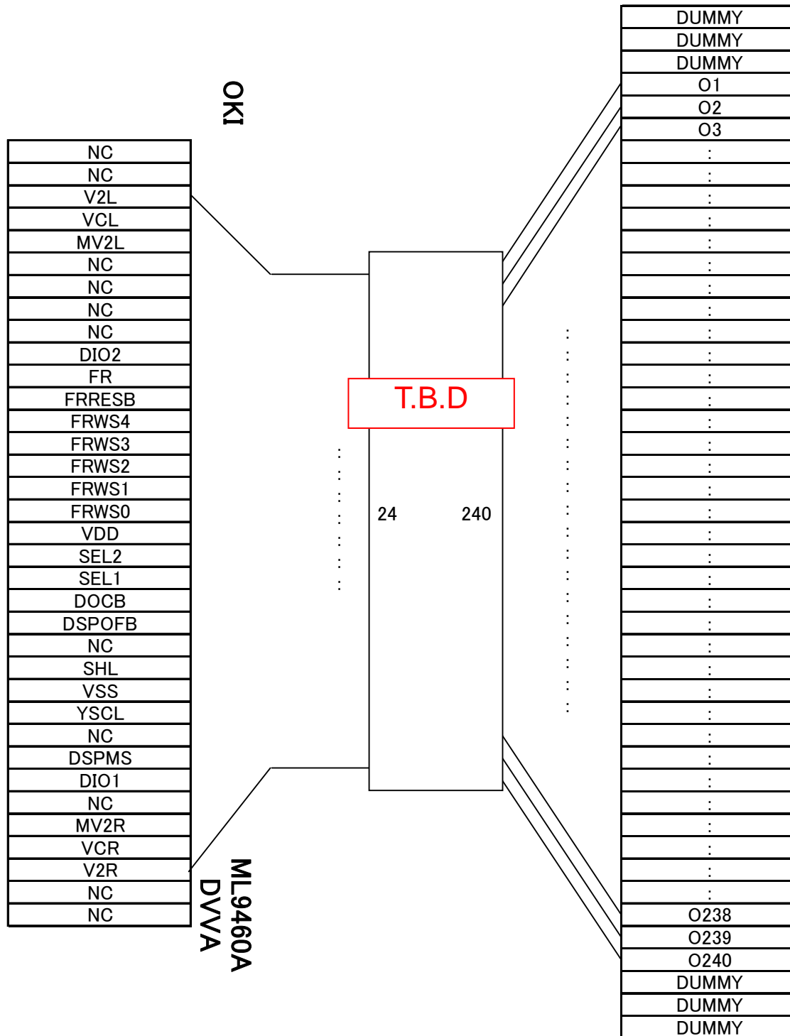
TOP VIEW
