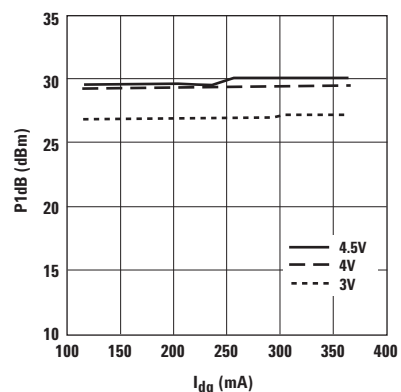
Figure 27. P1dB vs. I_{dq} and V_{ds} at 2 GHz.
