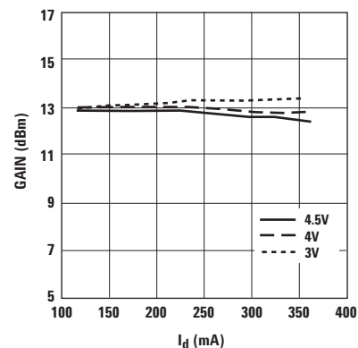
Figure 30. Gain vs. I_{ds} and V_{ds} at 2 GHz.
