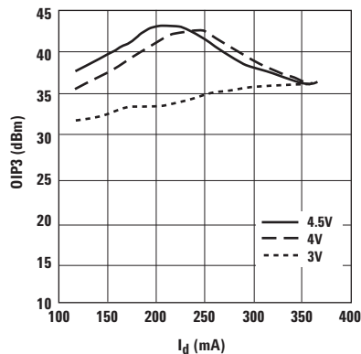
Figure 9. OIP3 vs. I_{ds} and V_{ds} at 900 MHz.
