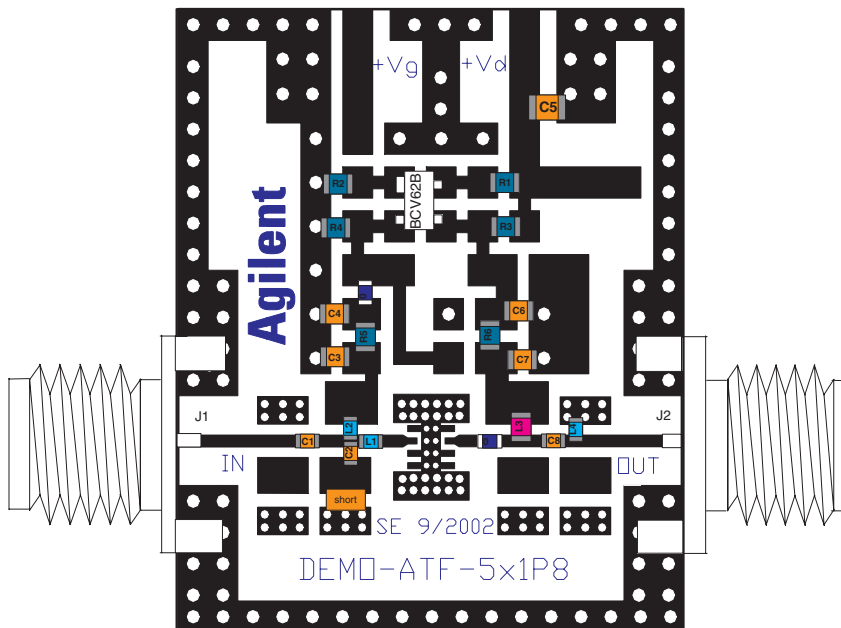
Figure 12. ATF-521P8 demoboard.
