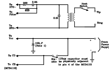
FIGURE 31.OPERATING FROM A POWER SUPPLY
