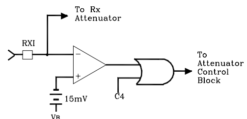
FIGURE 5.DIAL TONE DETECTOR
