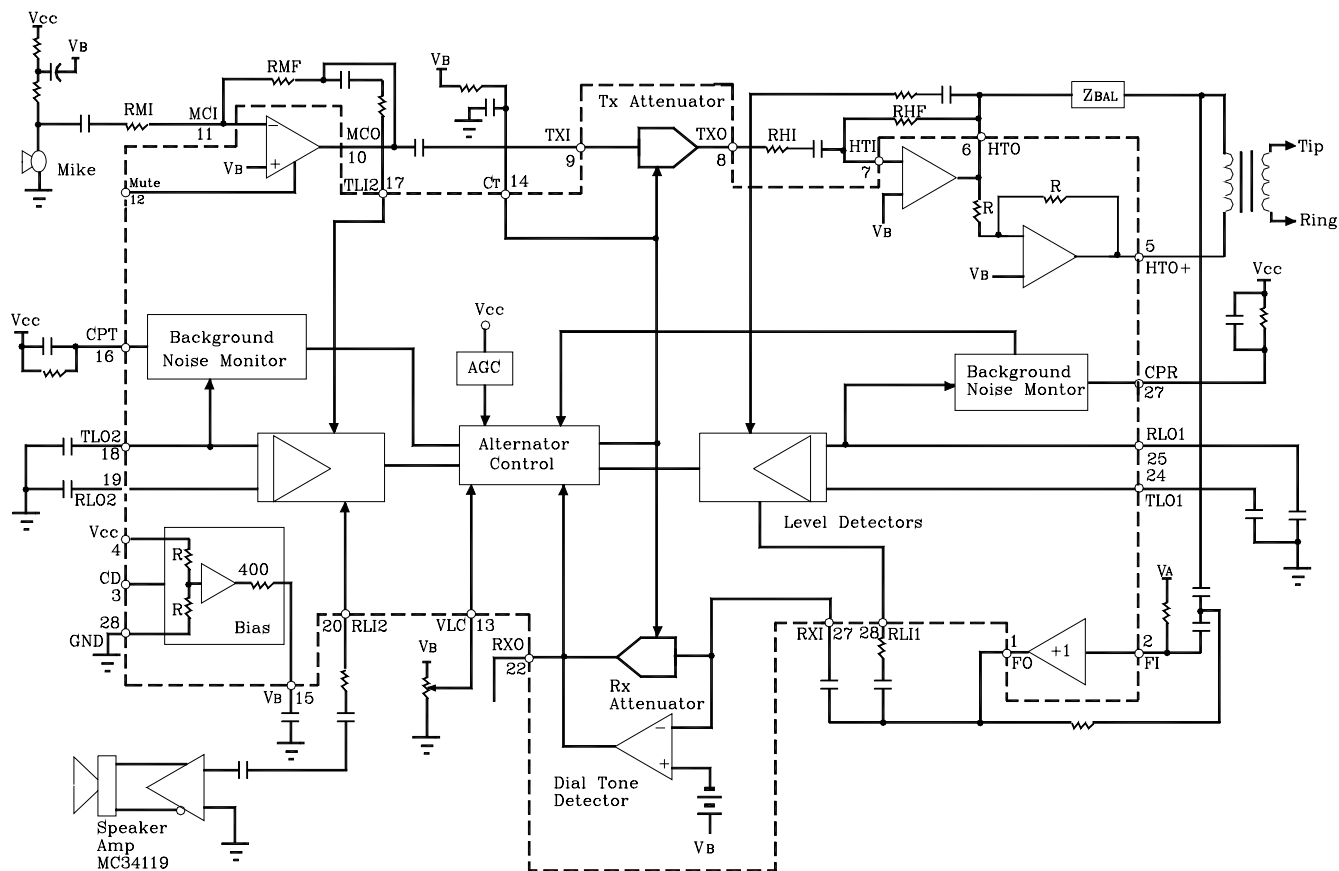
FIGURE 2.PJ34118 BLOCK DIAGRAM
