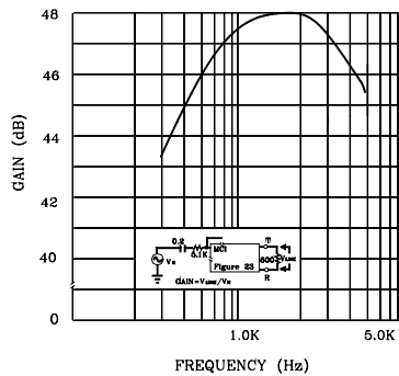
FIGURE 30.RECEIVE GAIN
