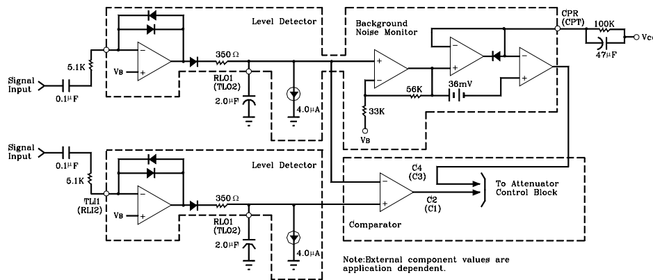
FIGURE 4.LEVEL DETECTORS
