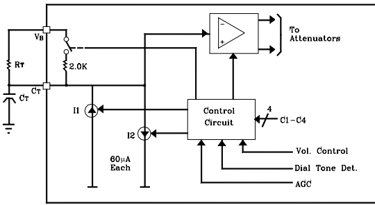
FIGURE 6. CT ATTENUATOR CONTROL BLOCK CIRCUIT
