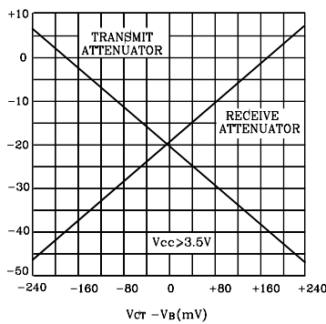
FIGURE 12.LEVEL DETECTOR AC TRANSFER CHARACTERISTICS
