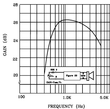
FIGURE 30.RECEIVE GAIN
