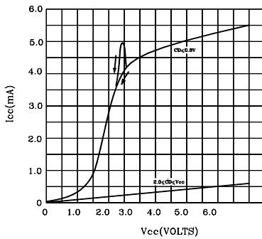
FIGURE 18. SUPPLY CURRENT versus SUPPLY VOLTAGE PUT CHARACTERISTICS
