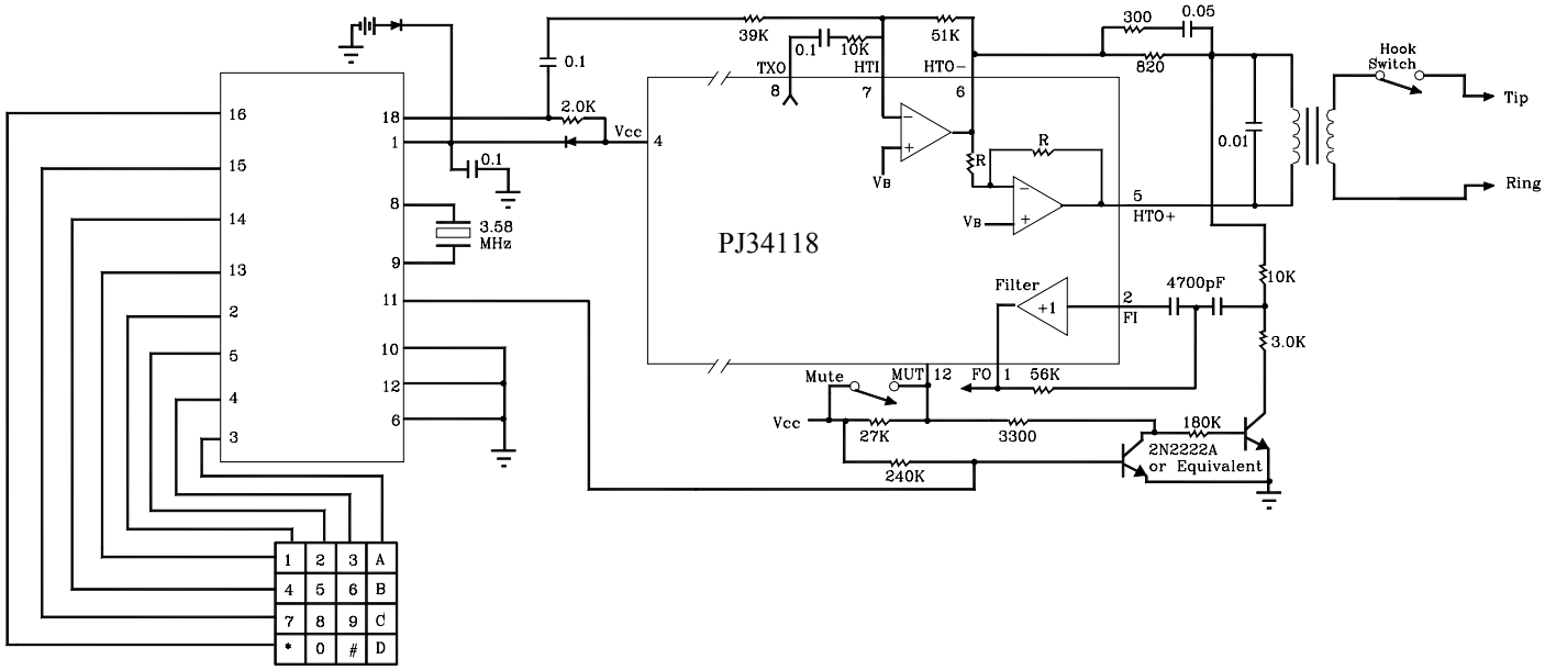
FIGURE 32.ADDING A DIALER TO THE SPEAKPHONE
