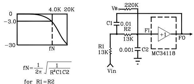
FIGURE 9. LOW PASS FILTER
