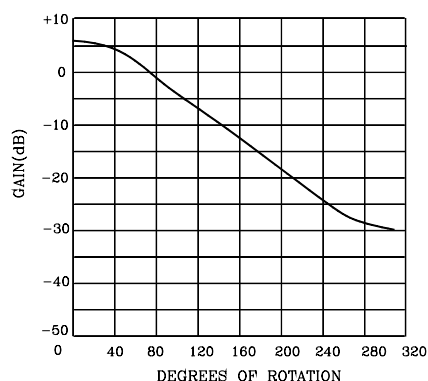
FIGURE 26. RECEIVE ATTENUATOR GAIN versus POTENTIOMETER POSITION USING AUDIO TAPER
