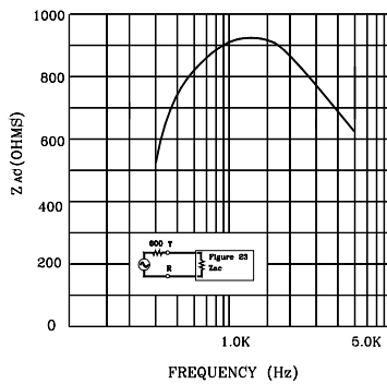
FIGURE 29.TRANSMIT GAIN-MICROPHONE TO TIP/RING
