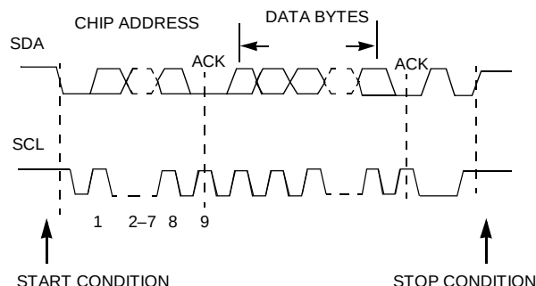
Figure 3. M_BUS Format
