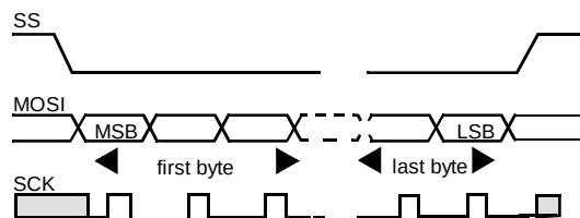
Figure 4. SPI Protocol
