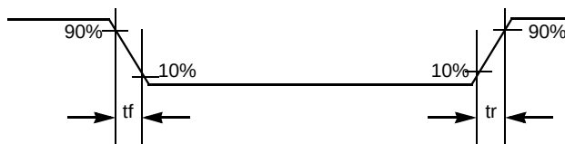
Figure 1. Switching Characteristics
