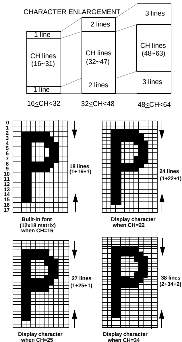
Figure 11. Variable Character Height
