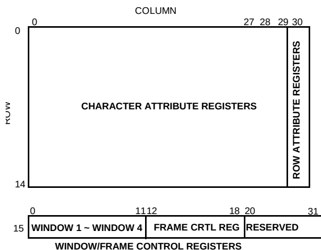
Figure 10. Memory Map of Attribute/Control Registers
