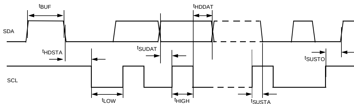
Figure 2. M_BUS TIMING
