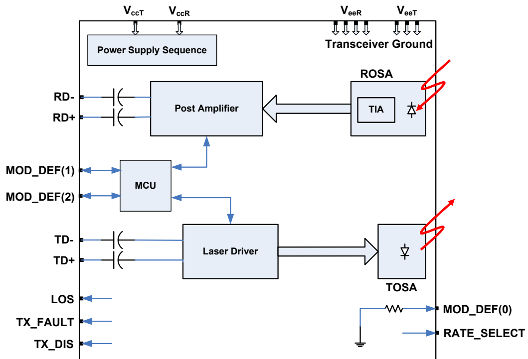
Figure 1 SFP optical transceiver functional block diagram
