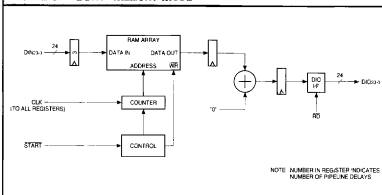
FIGURE 5. DELAY MEMORY MODE
