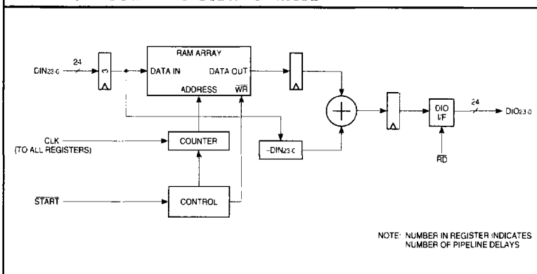
FIGURE 6. DELAY AND SUBTRACT MODE
