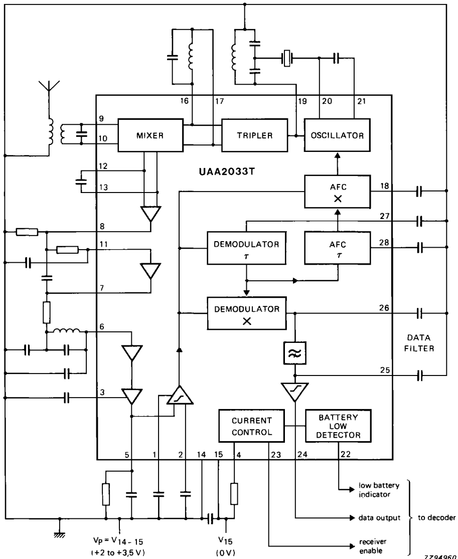
Fig. 1 Block diagram.
