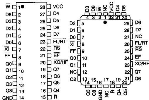
28-Pin DIP (600 Mil) See Mech. Drawing Pg. 966
