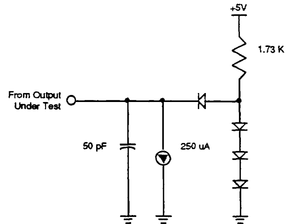
Figure 54. Standard Test Load
