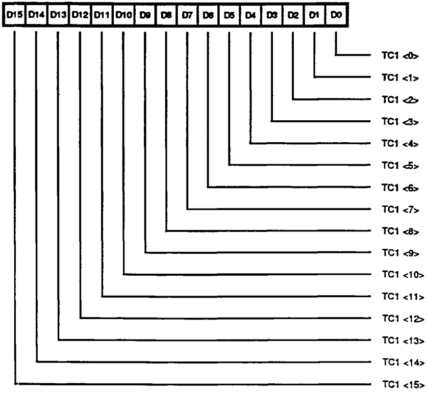
Figure 50. Time Constant 1 Register
