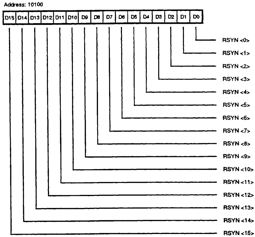
Figure 39. Receive Sync Register
