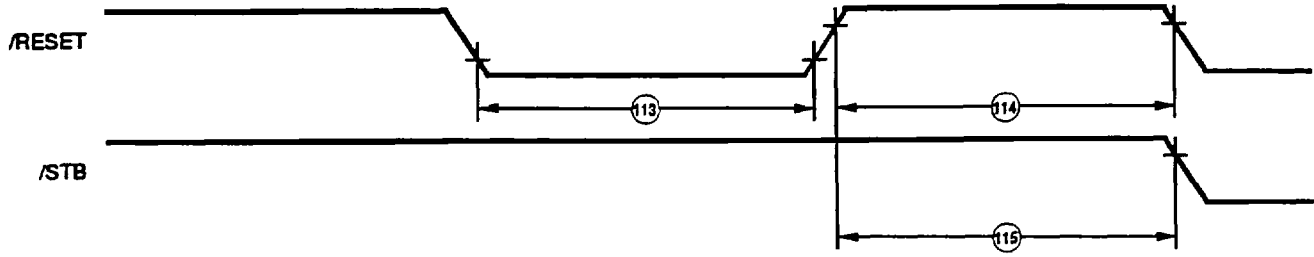
Figure 55. Reset Timing
