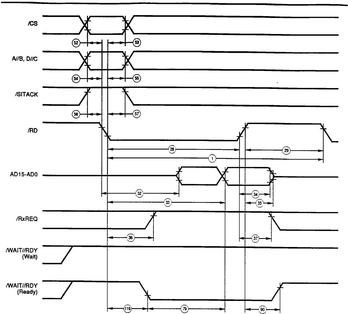
Figure 65. Non-Multiplexed /RD Read Cycle
