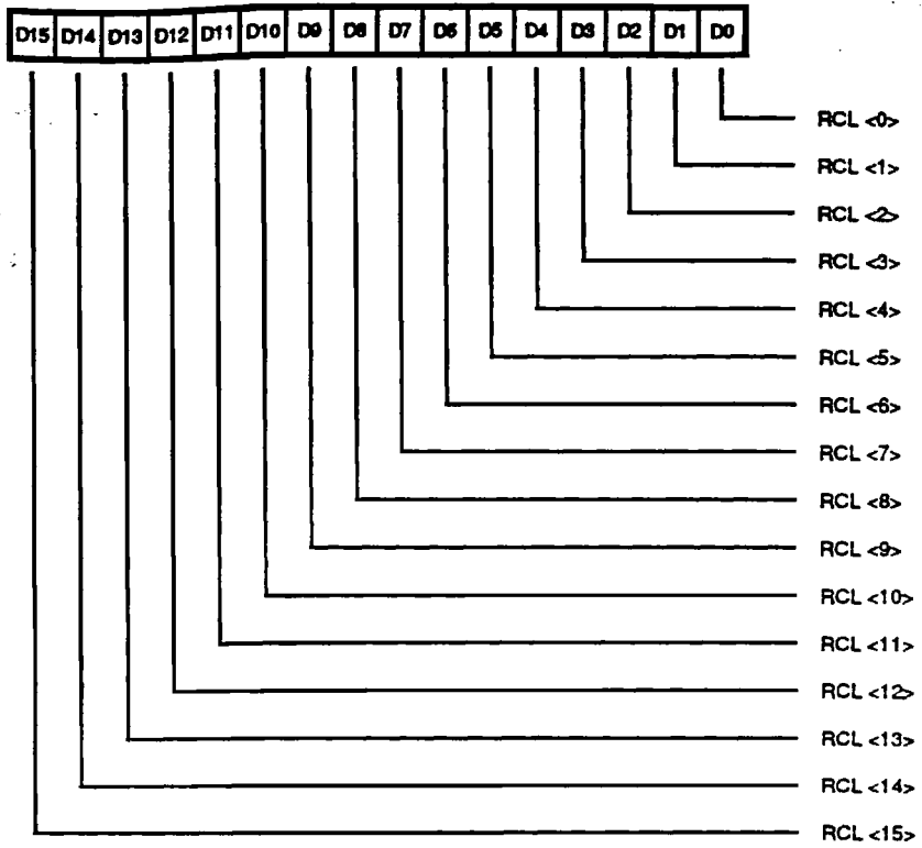
Figure 40. Receive Count Limit Register
