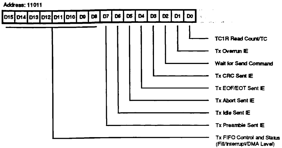
Figure 46. Transmit Interrupt Control Register
