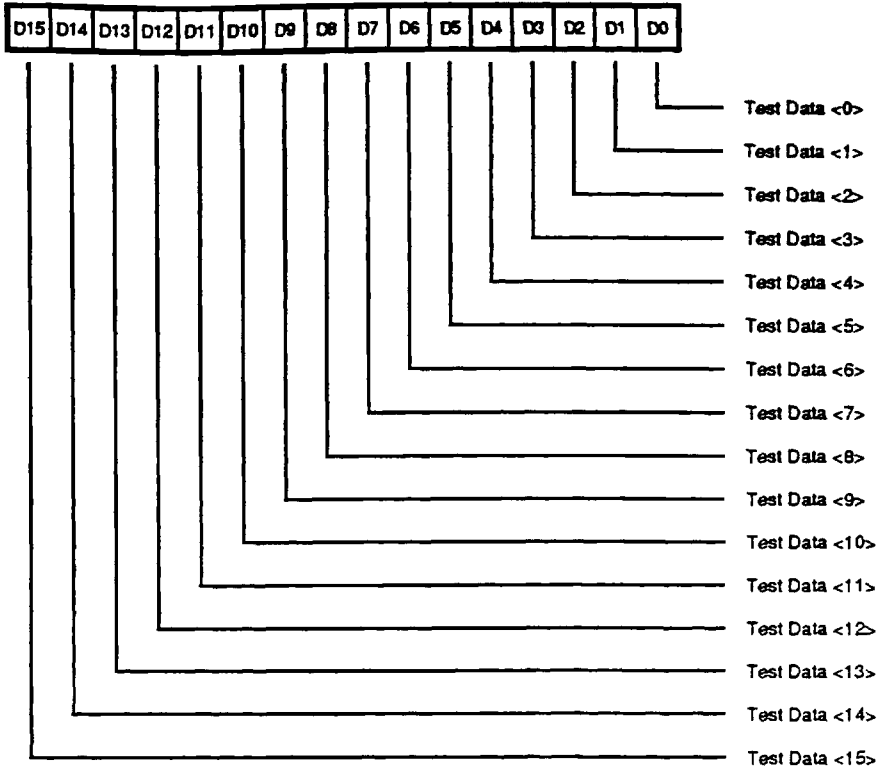
Figure 25. Test Mode Data Register
