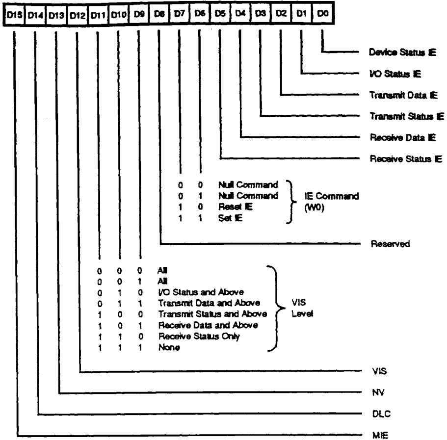
Figure 31. Interrupt Control Register
