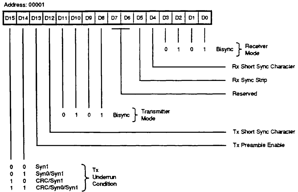
Figure 14. Channel Mode Register, Bisync Mode
