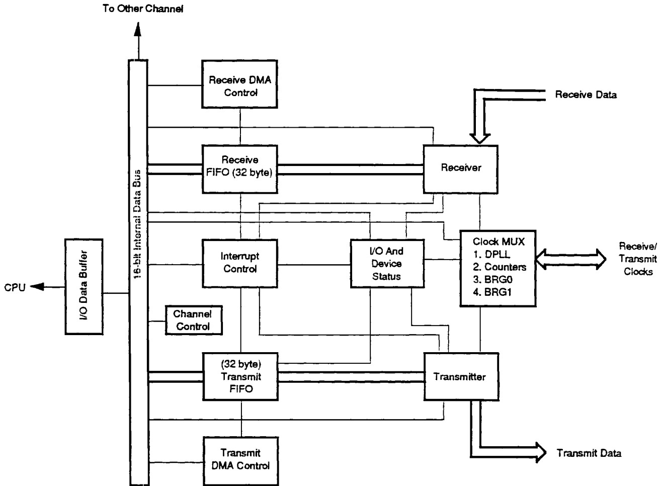
Figure 1. USC Block Diagram
