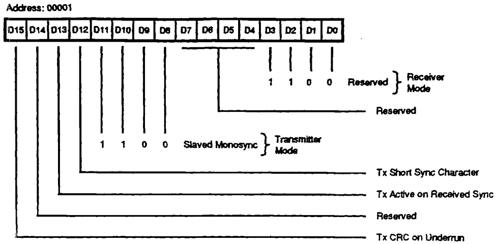
Figure 19. Channel Mode Register, Slaved Monosync Mode
