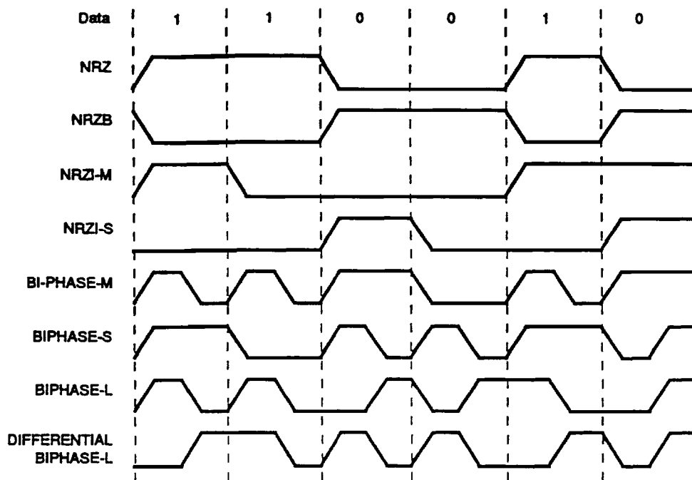
Figure 5. Data Encoding
