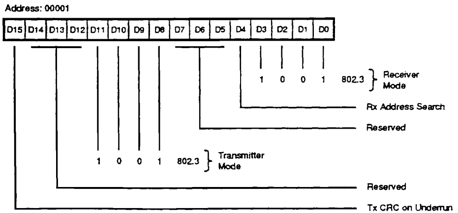
Figure 18. Channel Mode Register, 802.3 Mode
