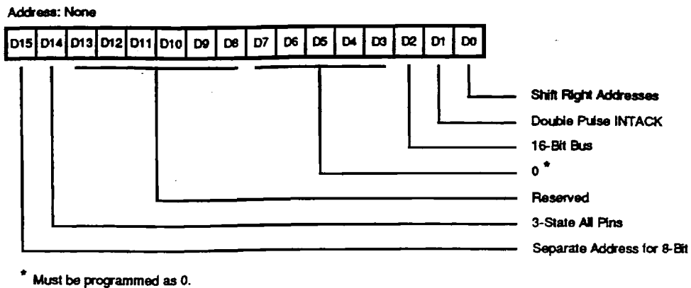
Figure 4. Bus Configuration Register
