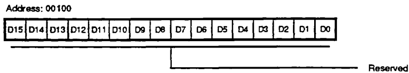
Figure 23. Primary Reserved Register
