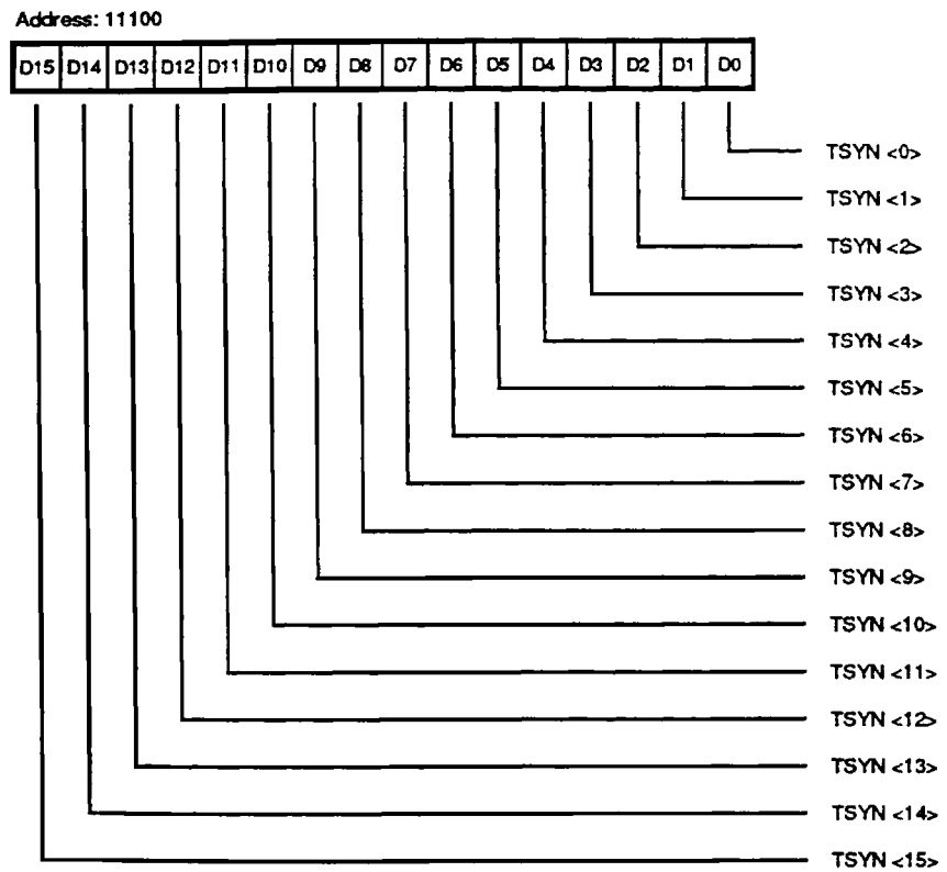
Figure 47. Transmit Sync Register
