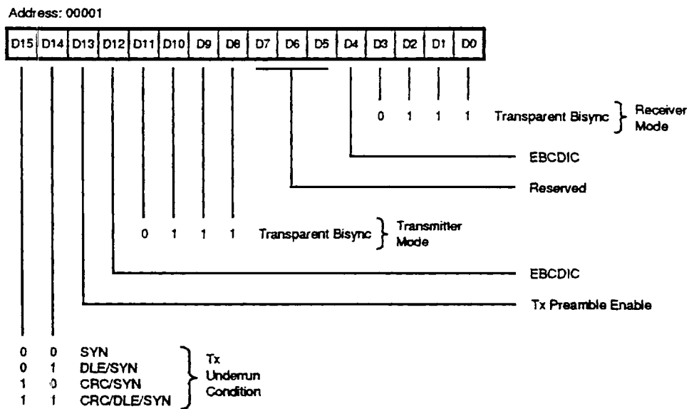
Figure 16. Channel Mode Register, Transparent Bisync Mode
