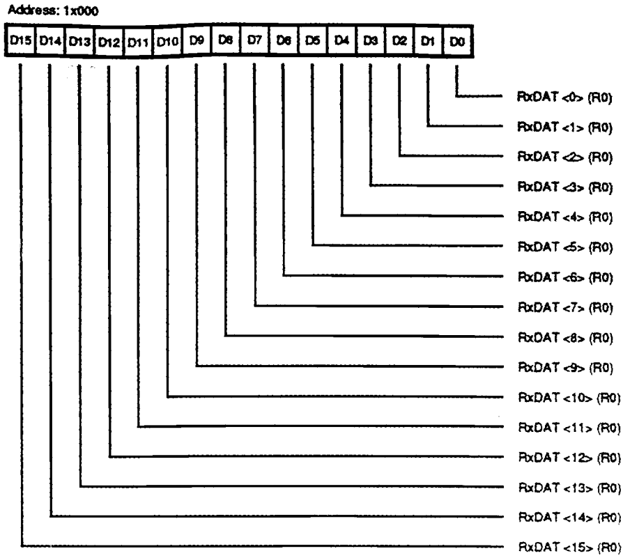
Figure 35. Receive Data Register
