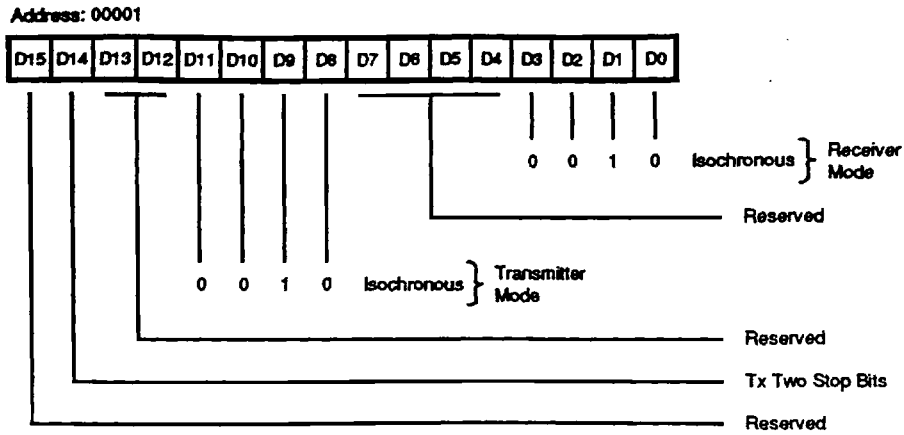
Figure 11. Channel Mode Register, Isochronous Mode
