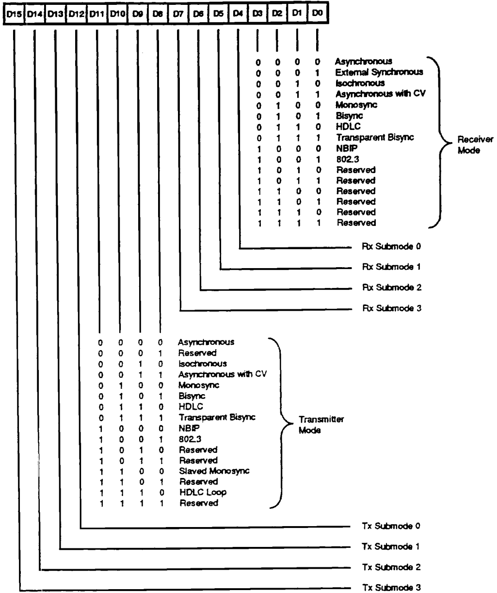
Figure 8. Channel Mode Register
