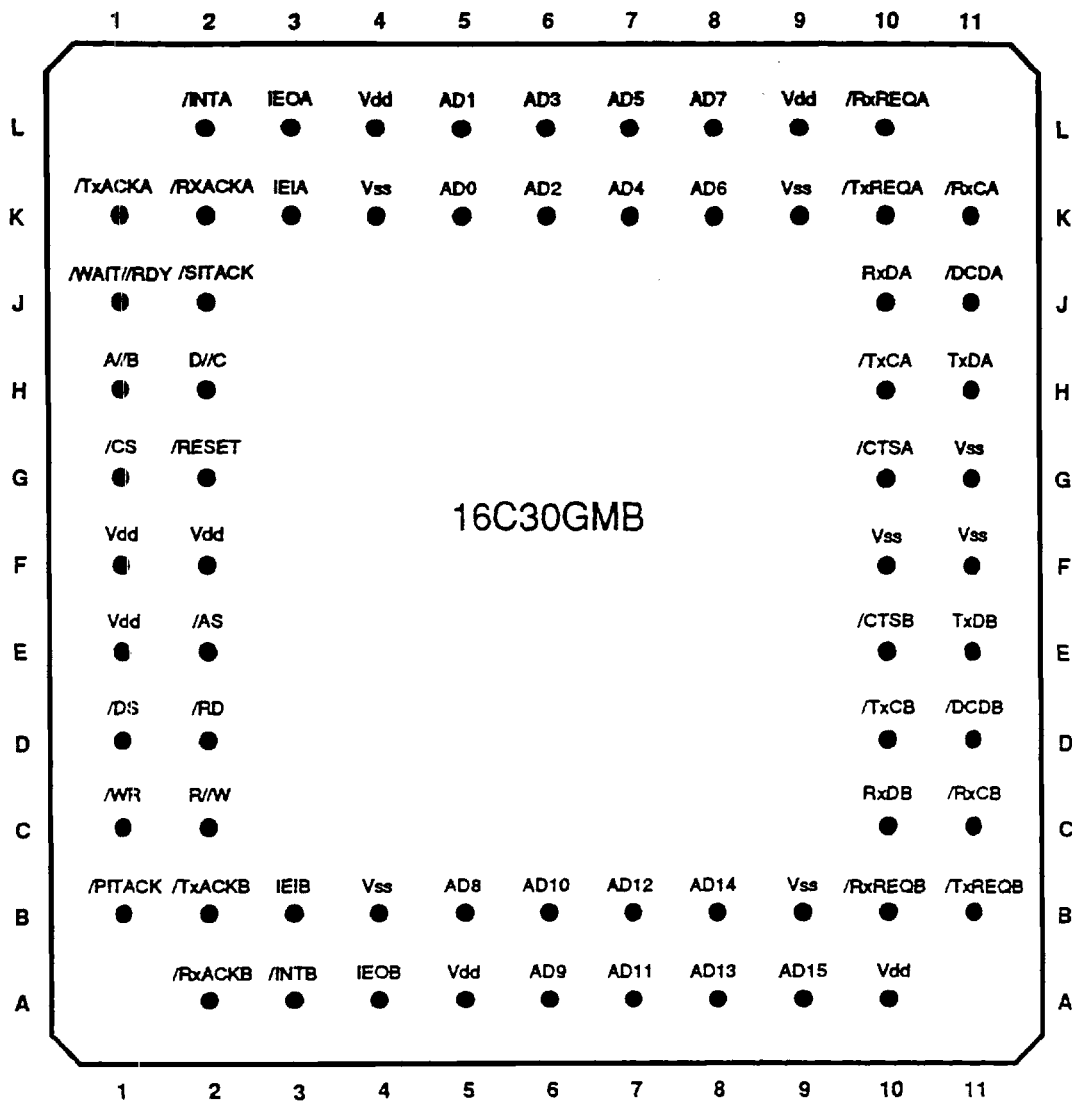
Figure 3. Pin Assignments
