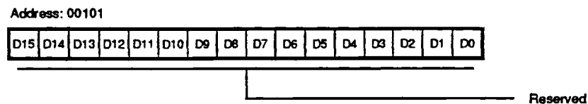
Figure 24. Secondary Reserved Register
