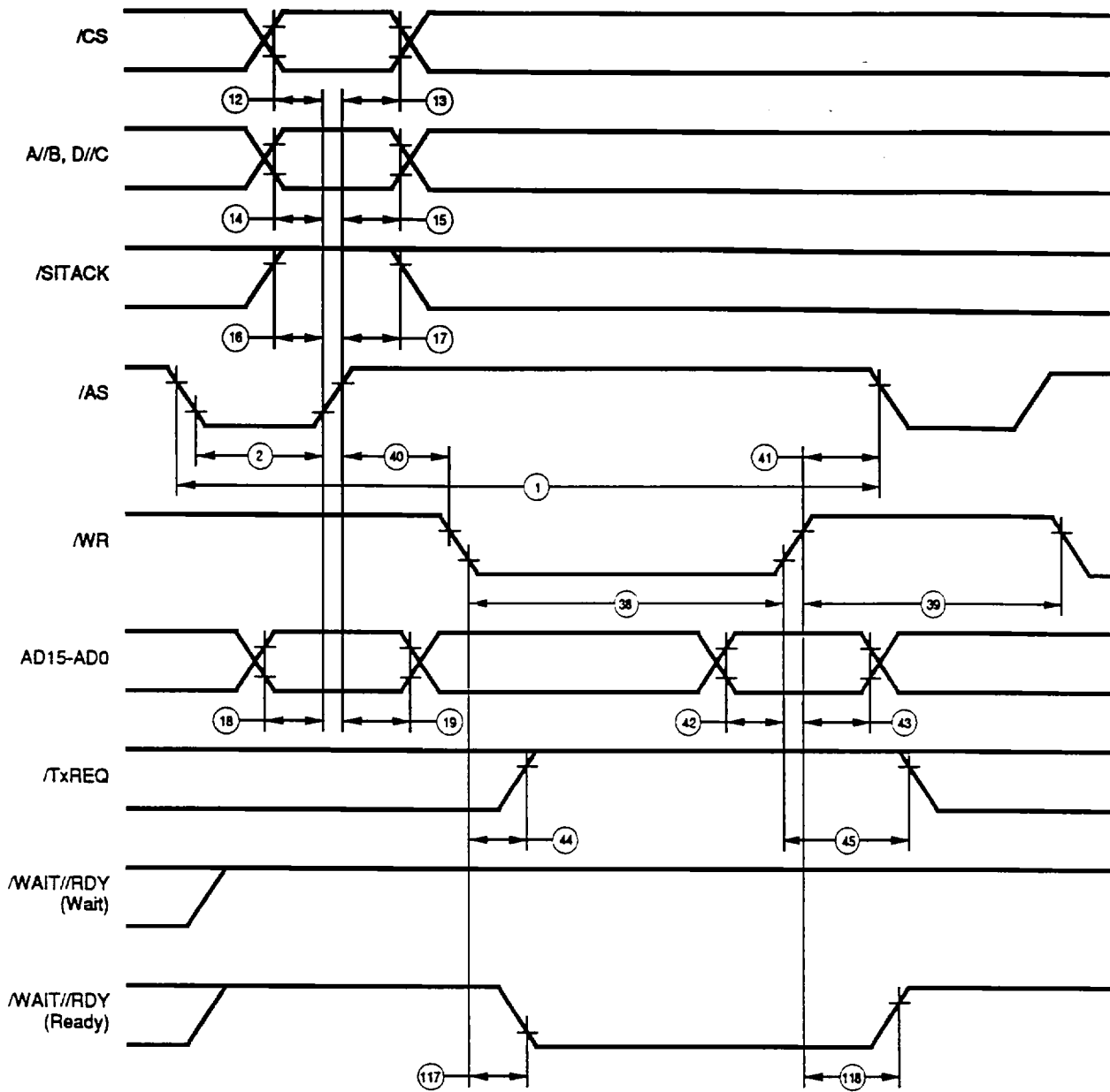
Figure 62. Multiplexed /WR Write Cycle
