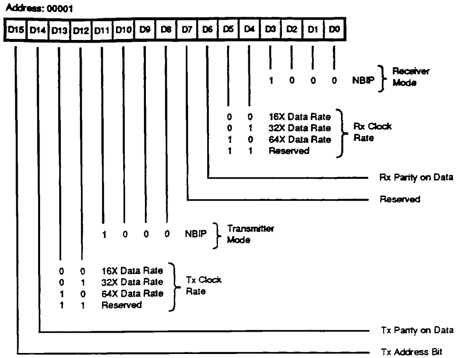
Figure 17. Channel Mode Register, NBIP Mode
