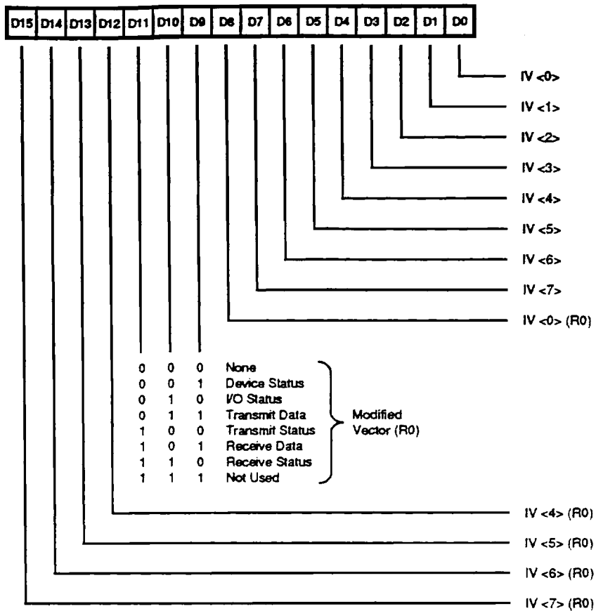
Figure 29. Interrupt Vector Register
