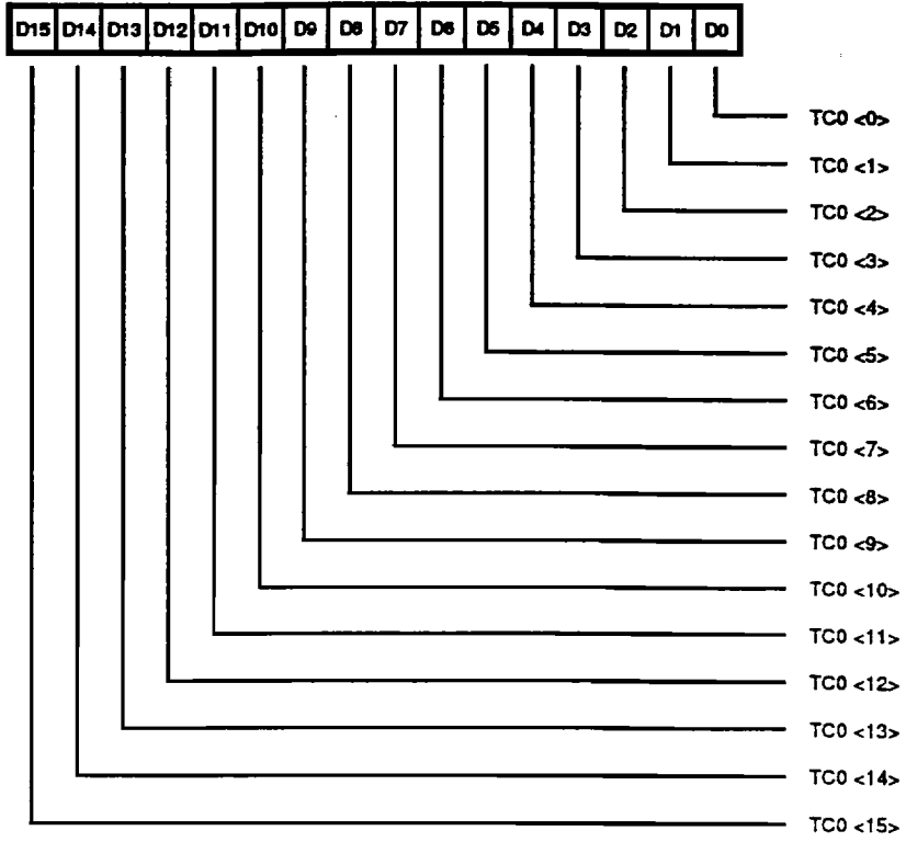
Figure 42. Time Constant 0 Register
