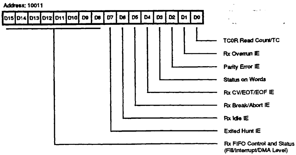
Figure 38. Receive Interrupt Control Register
