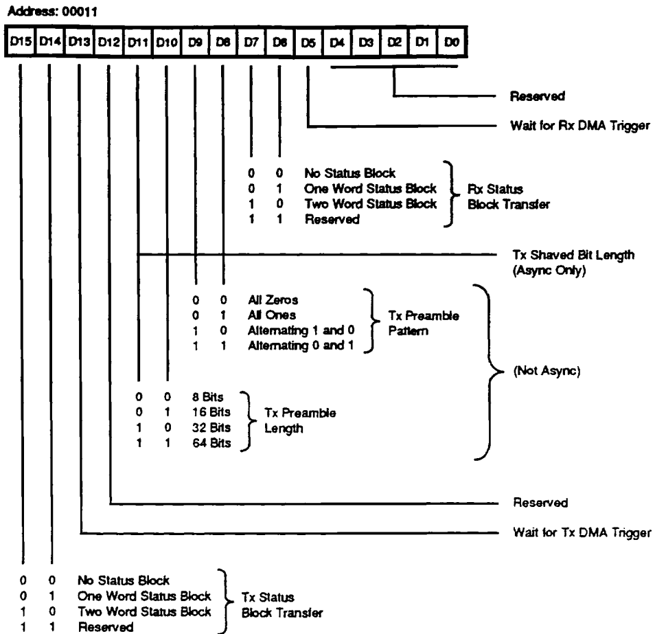
Figure 22. Channel Control Register
