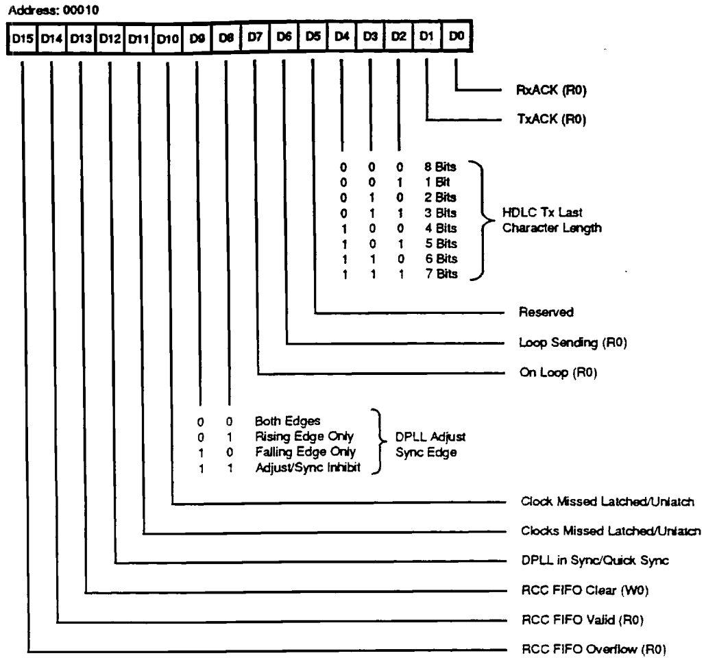
Figure 21. Channel Command/Status Register
