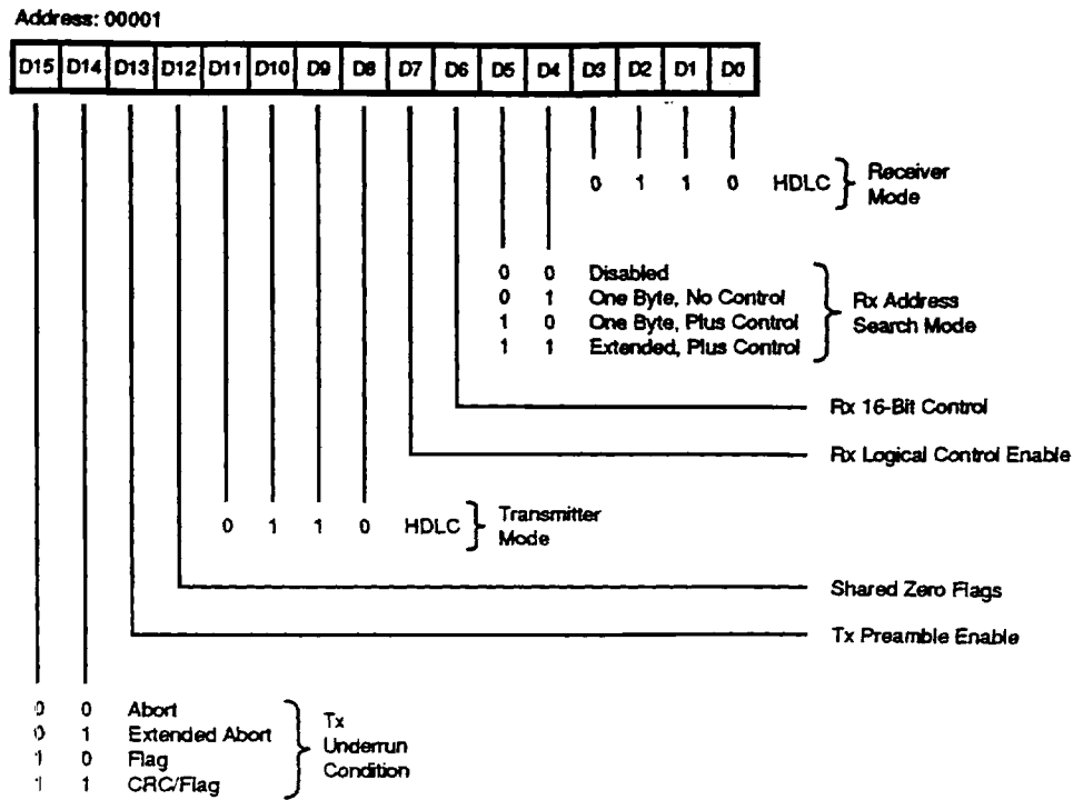
Figure 15. Channel Mode Register, HDLC Mode
