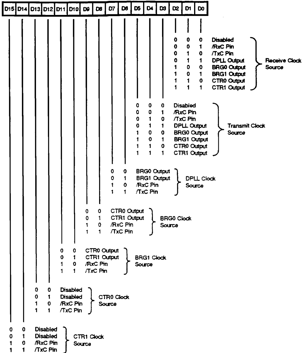
Figure 27. Clock Mode Control Register
