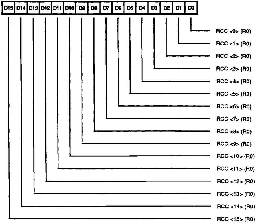
Figure 41. Receive Character Count Register
