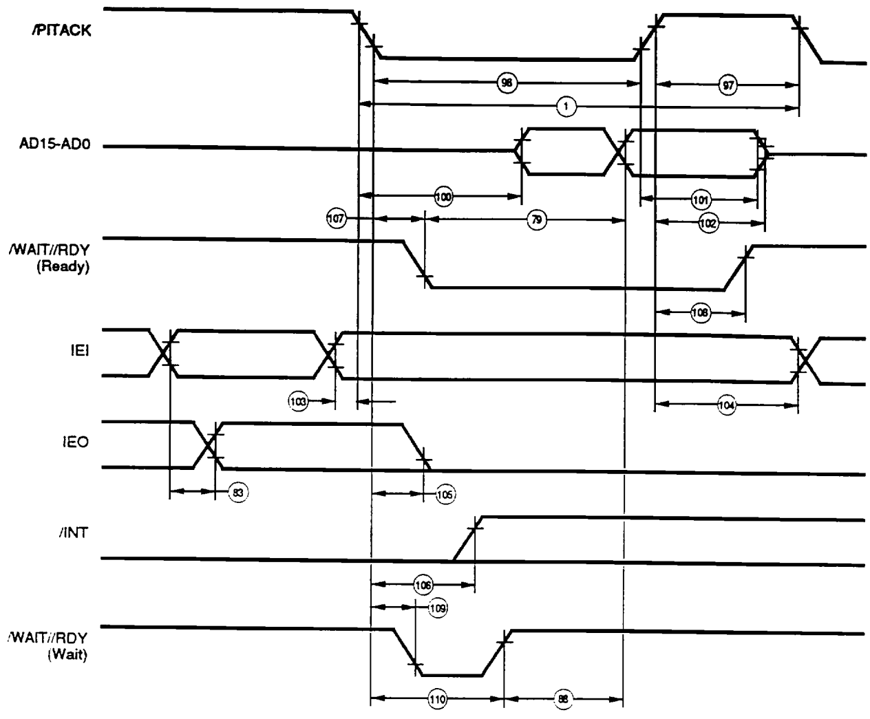
Figure 72. Non-MUX /RD Interrupt Acknowledge Cycle
