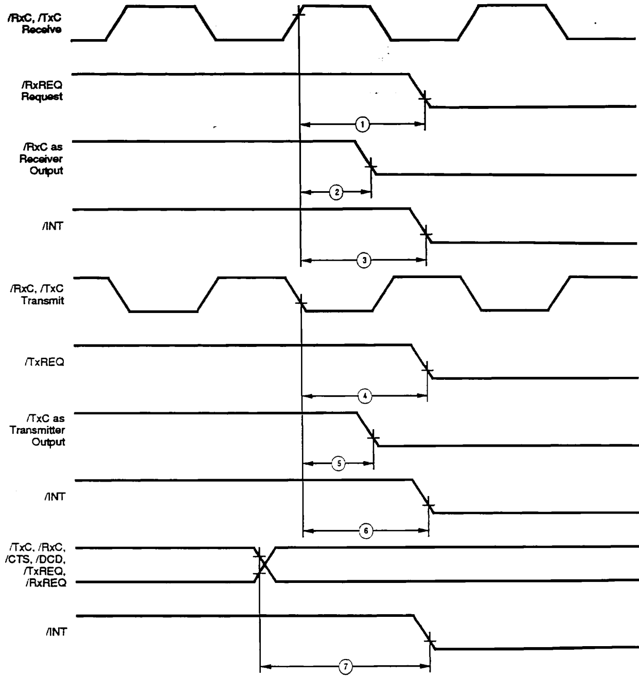
Figure 76. Z16C30 System Timing
