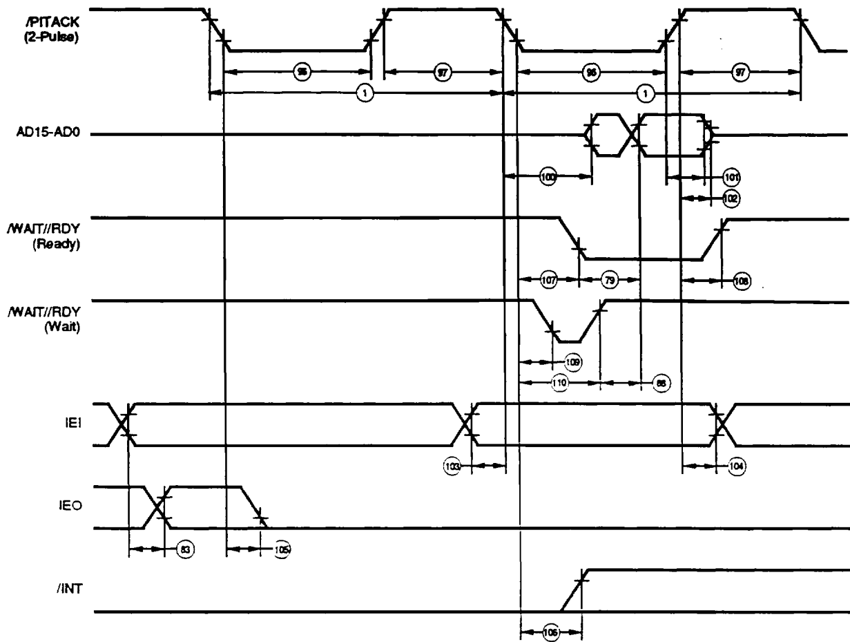
Figure 74. Non-Multiplexed Double-Pulse Intack Cycle
