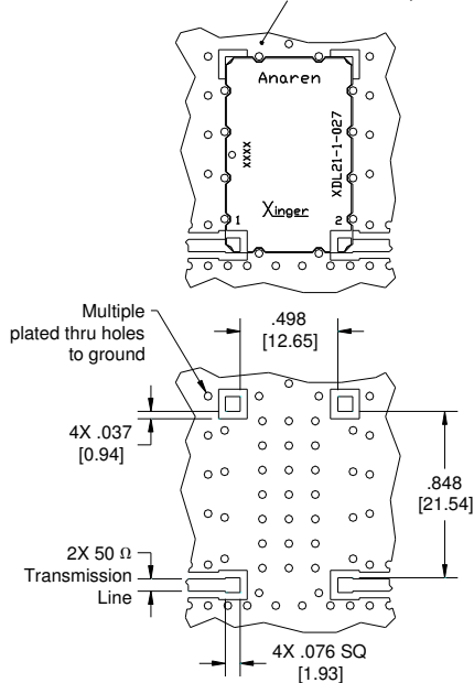
Dimensions are in Inches [Millimeters] XDL21-1-027 Mounting Footprint
