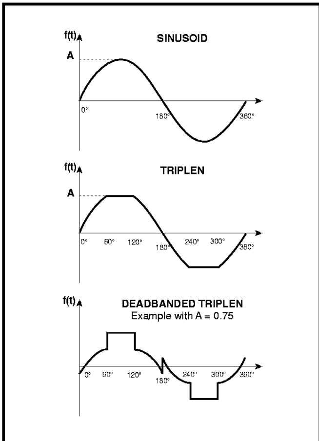
Fig.14 Power waveforms
