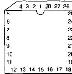
PLCC-28 (TOP VIEW) QP PACKAGE
