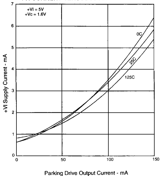
+VI CURRENT VERSUS PARK DR CURRENT
