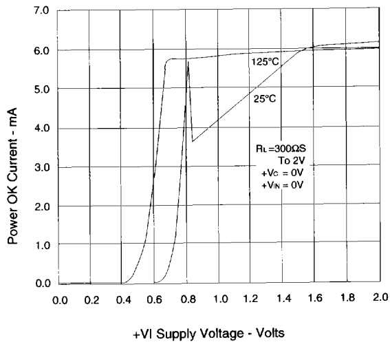
POWER OK CURRENT vs. +VI SUPPLY
