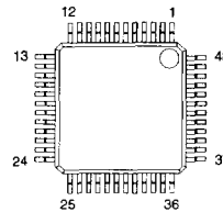
TQFP-48 (TOP VIEW) FQ PACKAGE
