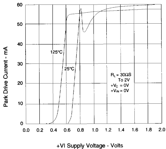
PARK DRIVE CURRENT vs. +VI SUPPLY
