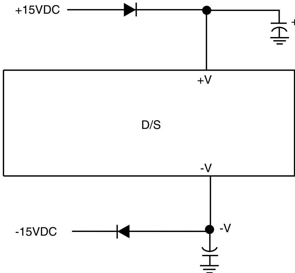
FIGURE 11. PROTECTION CIRCUITRY
