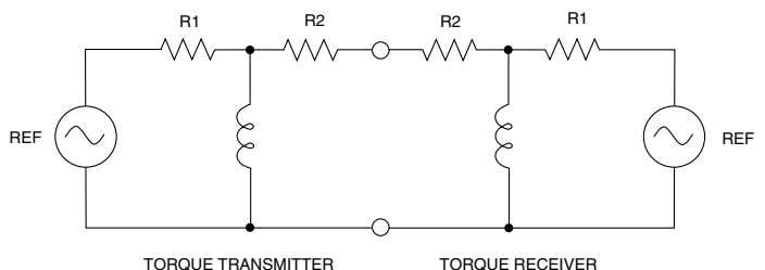
FIGURE 6. TORQUE SYSTEM
