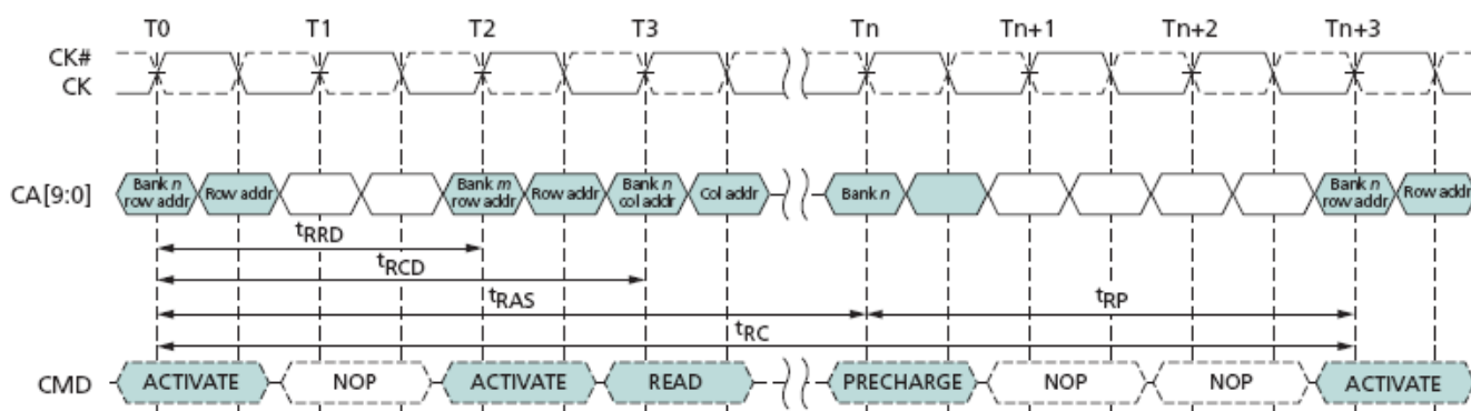
Activate command cycle: t RCD=3, t RP=3, t RRD=2
