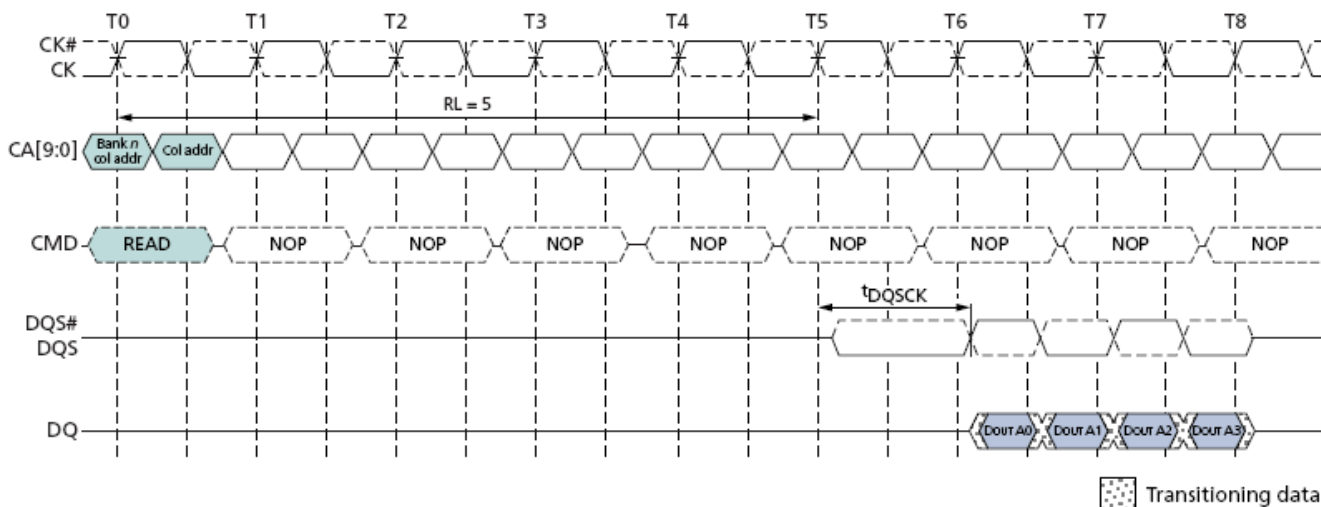
Burst Read: RL=5, BL=4, t_{DQSC} > t_{CK}
