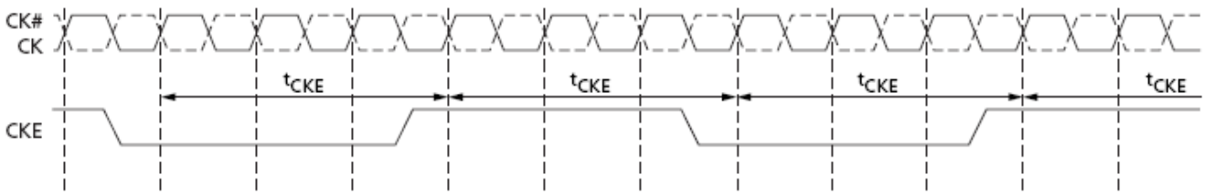
CKE intensive environment
