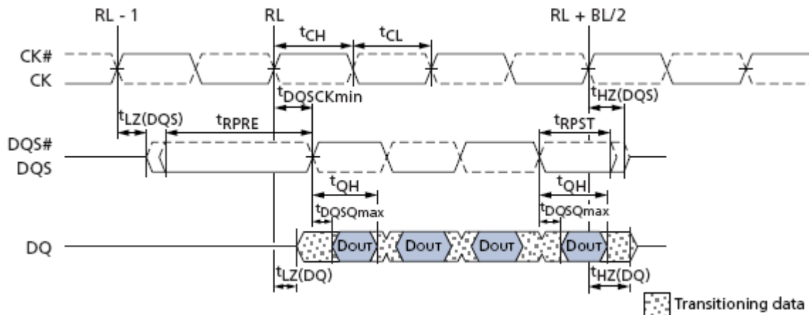
Data output (Read) timing ( t_{DQSCmin} ), BL=4
