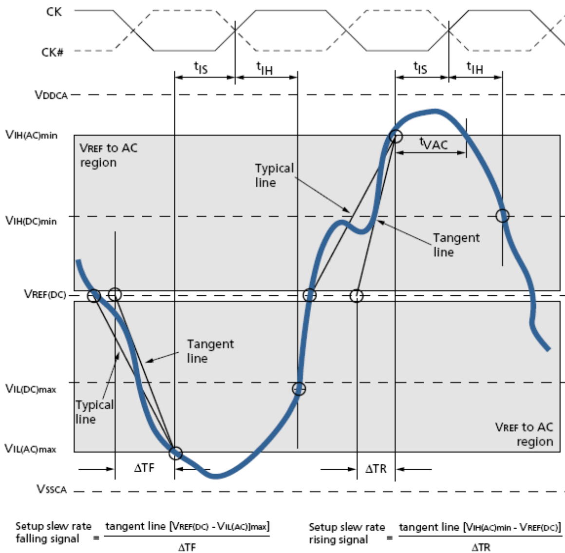
Tangent Line: t_{IS} for CA and \overline{CS} Relative to Clock
