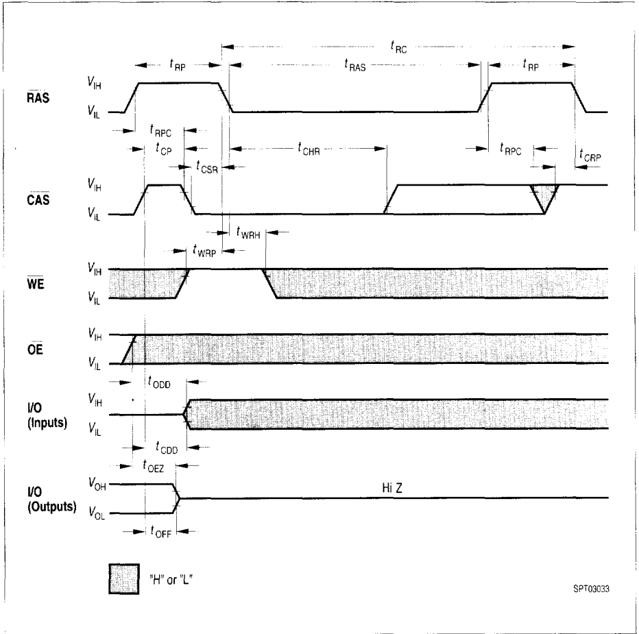
CAS-before-RAS Refresh Cycle
