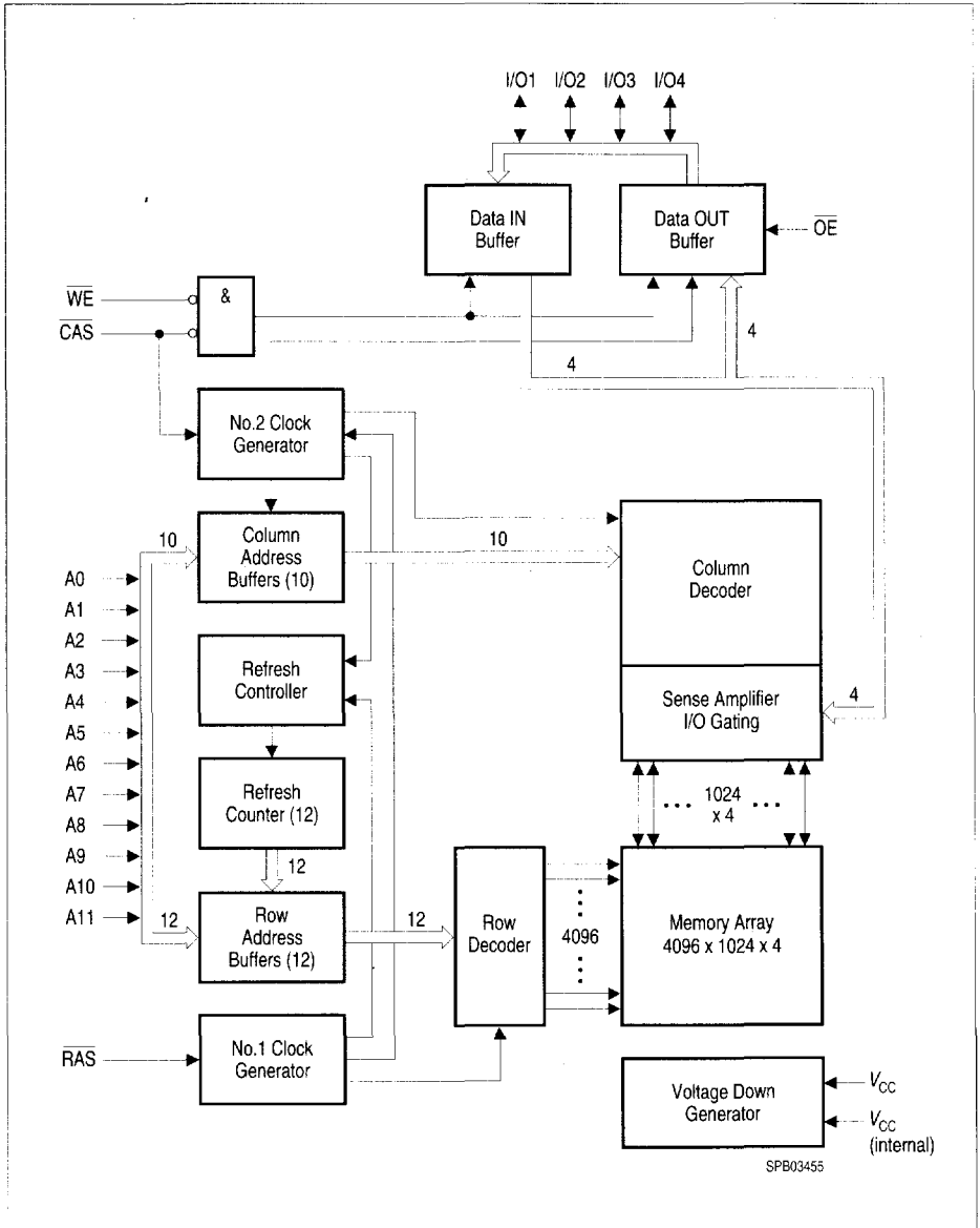
Block Diagram for HYB 5(3)116405 (4k-refresh)
