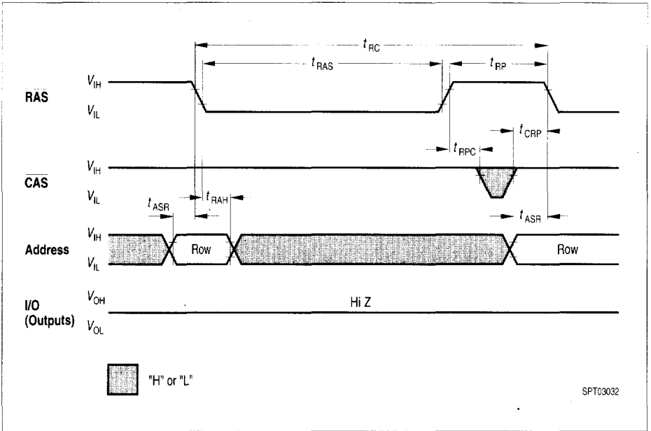
RAS-only Refresh Cycle
