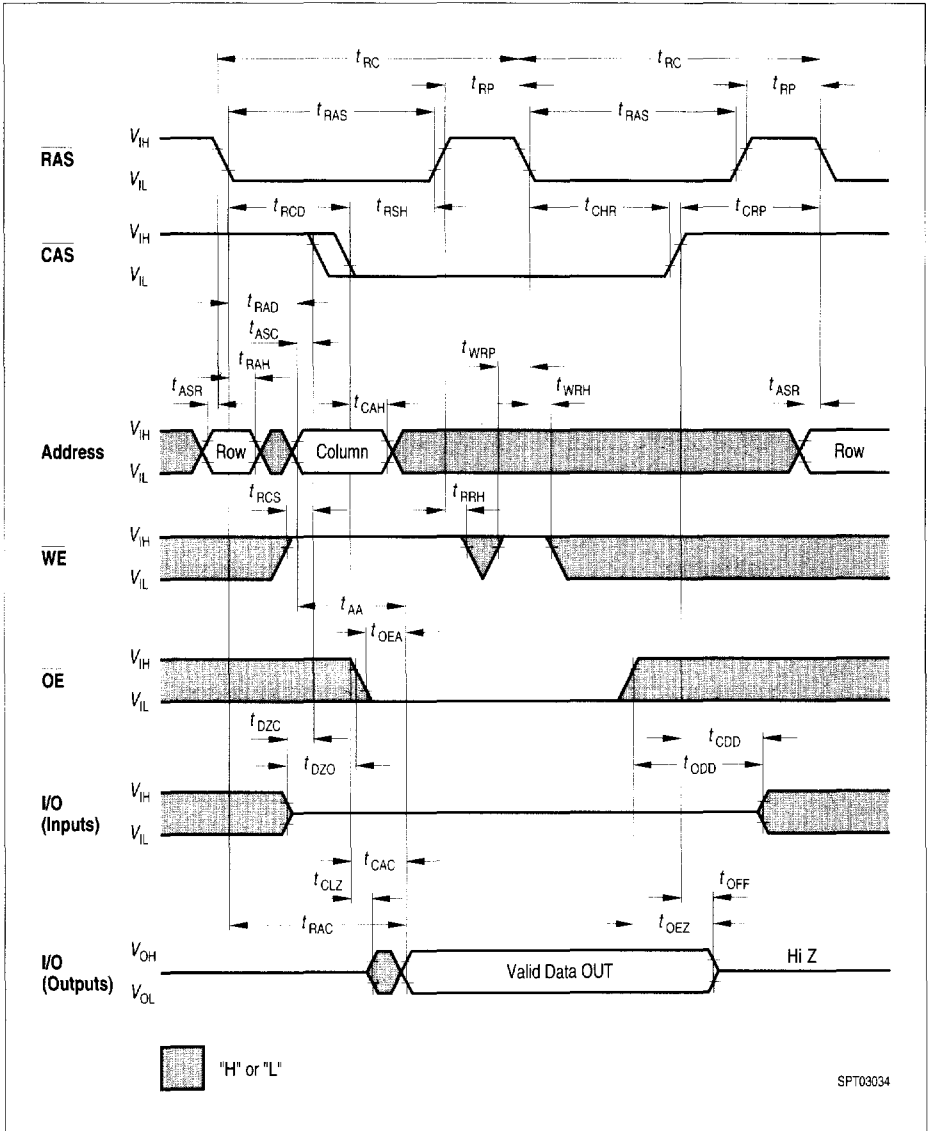
Hidden Refresh Cycle (Read) Cycle
