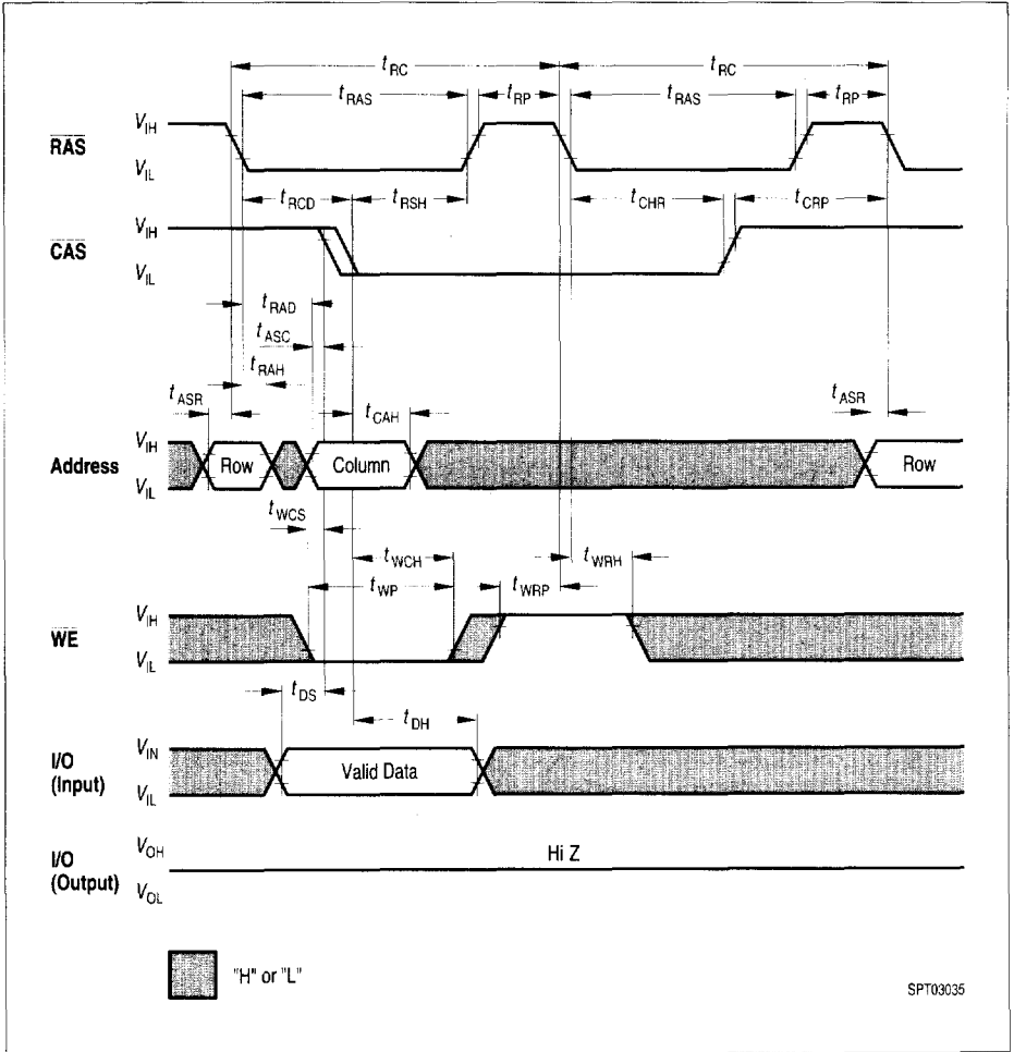
Hidden Refresh Early Write Cycle
