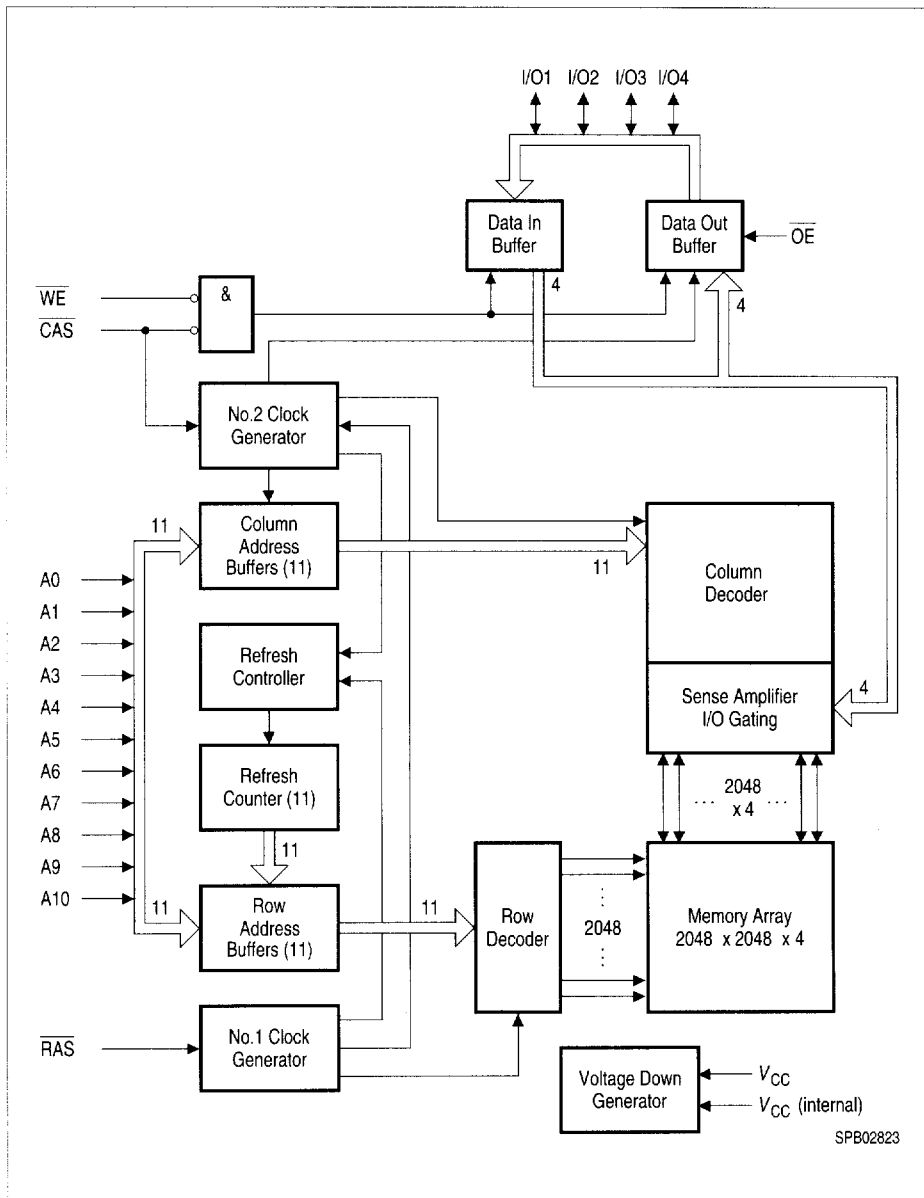
Block Diagram for HYB 5(3)117405 (2k-refresh)
