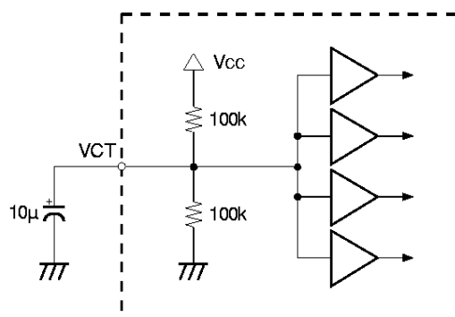
Fig. 8. VCT Buffer
