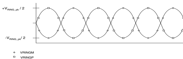
Figure 5. Ringing Waveforms
