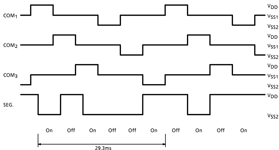
Fig.15 LCD drive waveform
