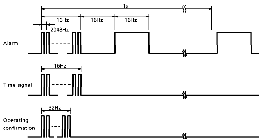
Fig.14 Buzzer drive waveform
