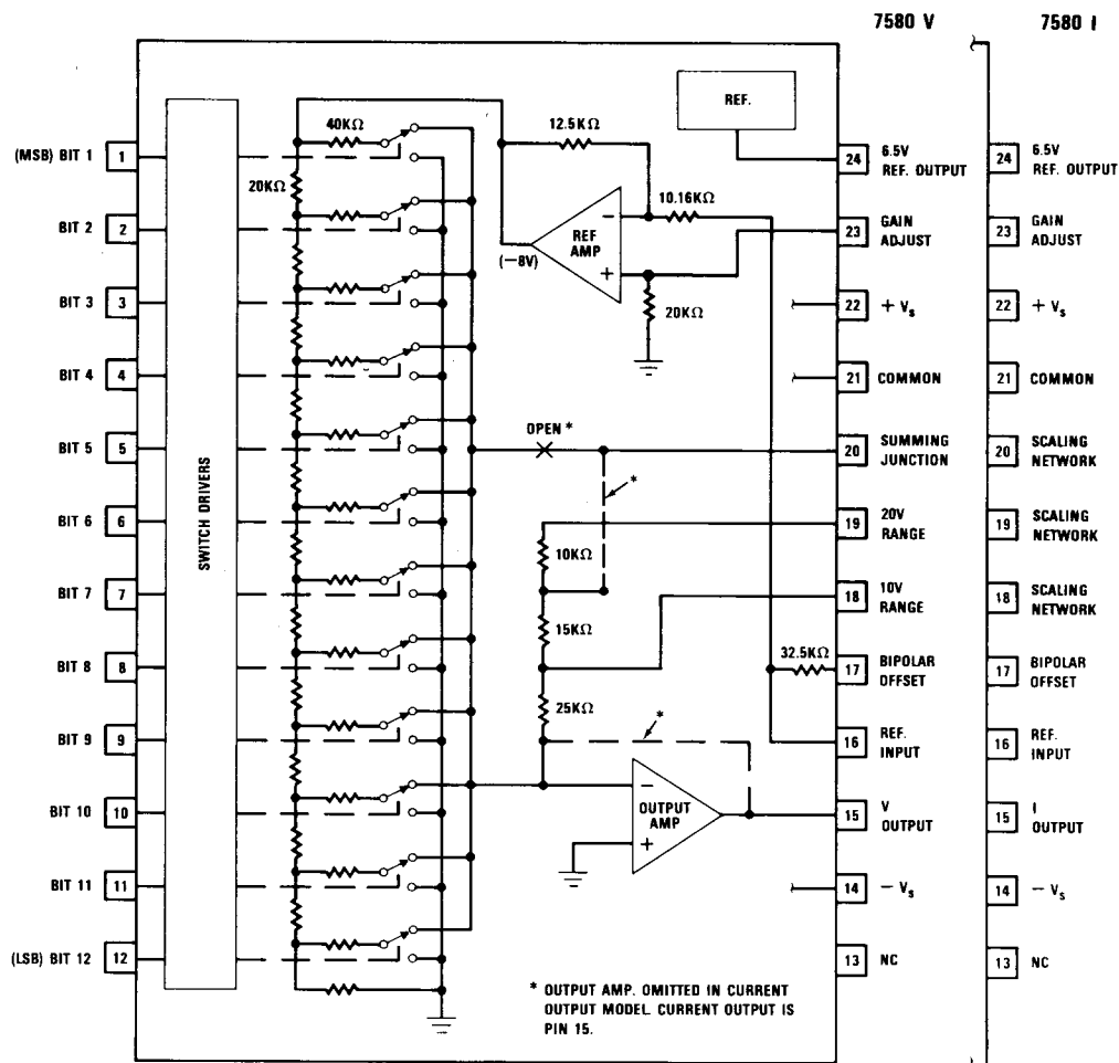
Figure 1. Series 7580 Block Diagram
