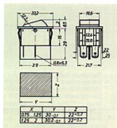
NON-ILLUMINATED, DOUBLE POLE R62 16A-125V AC, 1/8 HP, 10A-250V AC, 1/3 HP
