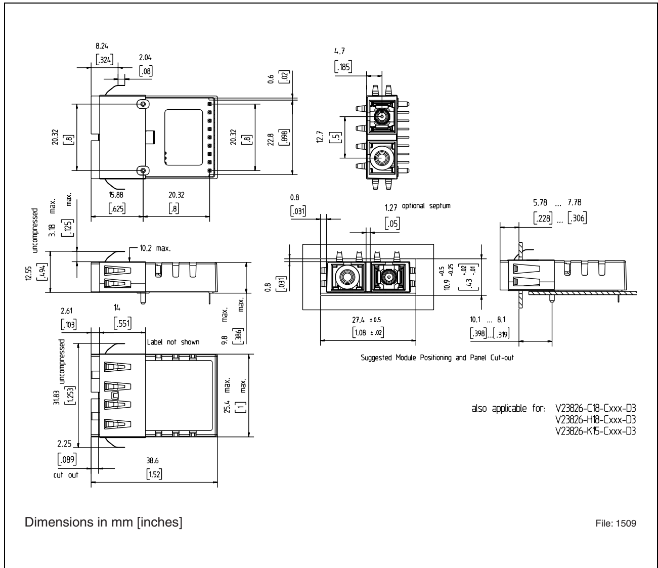
Figure 7 Shield with Backward Springs, -D3
