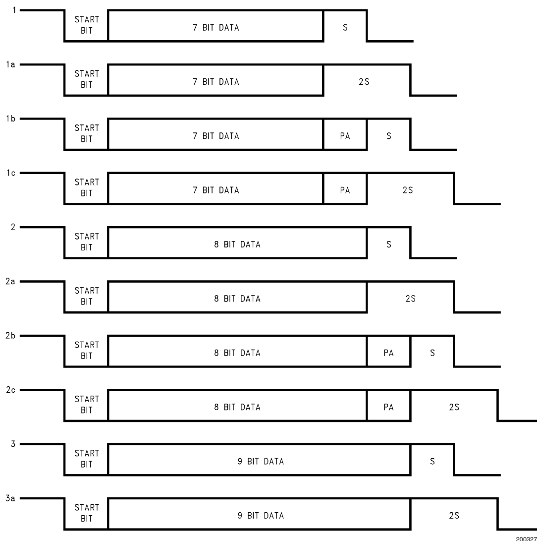
FIGURE 23. Framing Formats
