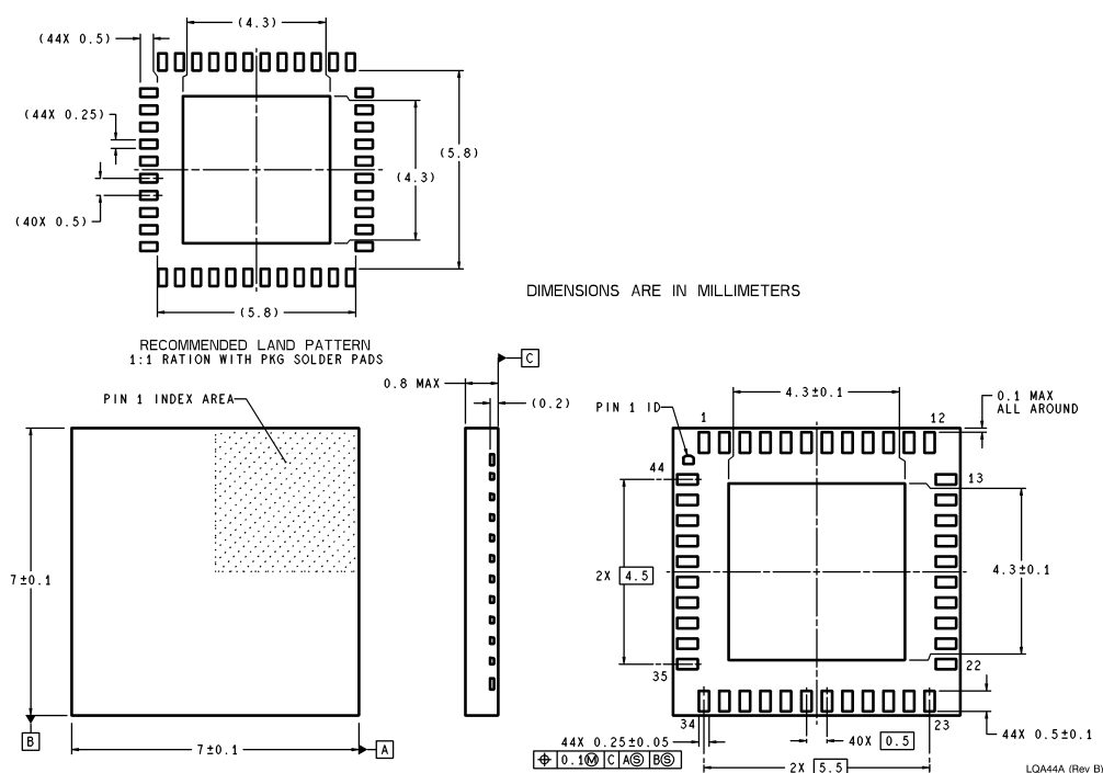
LLP Package (LQA) Order Number COP8SBE9HLQ7, COP8SCE9HLQ7 or COP8SCE9HLQ9 NS Package Number LQA44A
