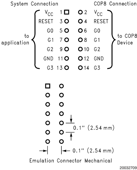
FIGURE 6. Emulation Connection
