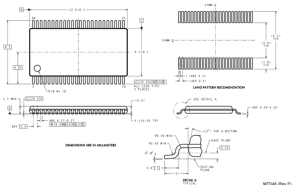
TSSOP Package (MTD) Order Number COP8SBE9IMT7, COP8SCE9IMT7 or COP8SCE9IMT9 NS Package Number MTD48
