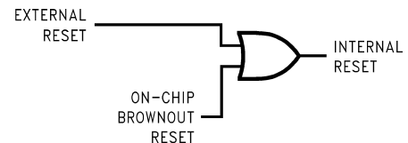
FIGURE 8. Reset Logic
