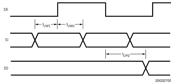
FIGURE 1. MICROWIRE/PLUS Timing
