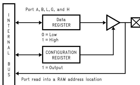
FIGURE 4. I/O Port Configurations—Output Mode
