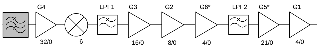
Figure 9. IF and I/Q Gain Distribution (dB)
