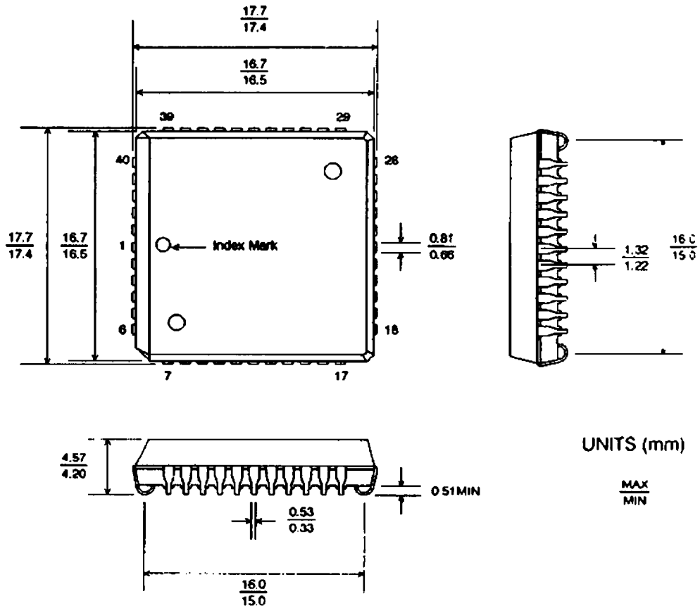
Figure 4. HBCR-1801, -1811, -2001, -2011
