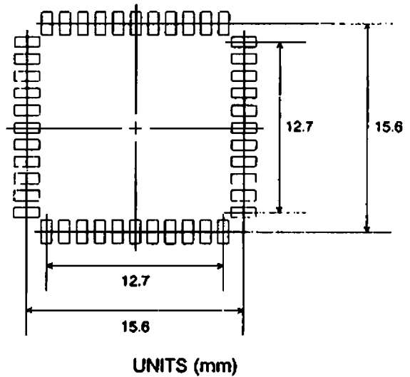
Figure 6. Pad Placement
