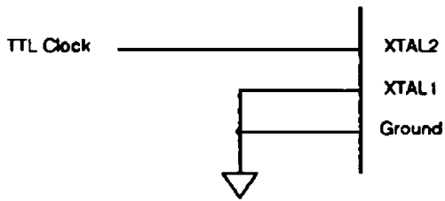
Figure 10. 1800, 1801, 2000, 2001 ICs
