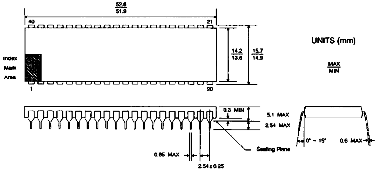
Figure 3. HBCR-1800, -1810, -2000, -2010
