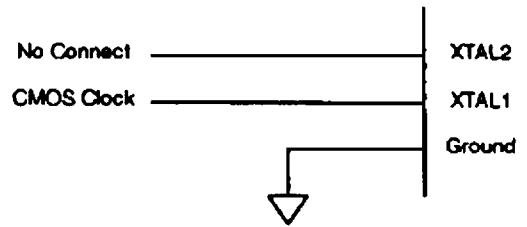
Figure 11. 1810, 1811, 2010, 2011 ICs
