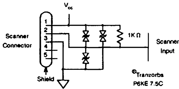
Figure 7. Recommended Interface
