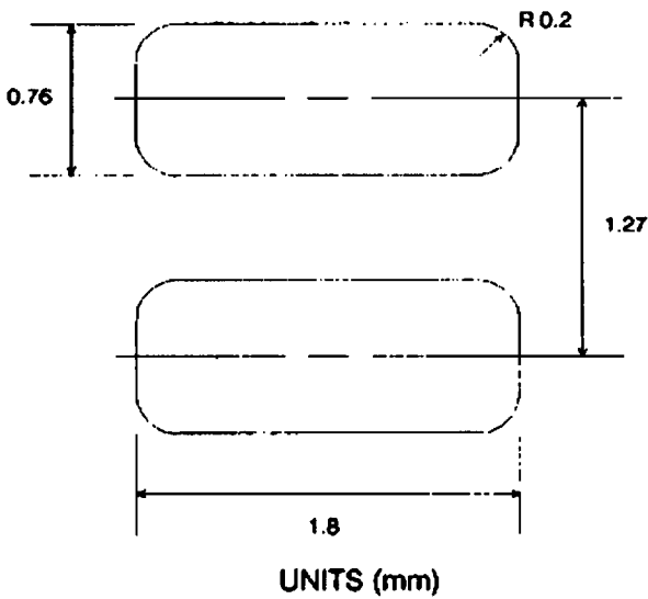
Figure 5. Pad Size
