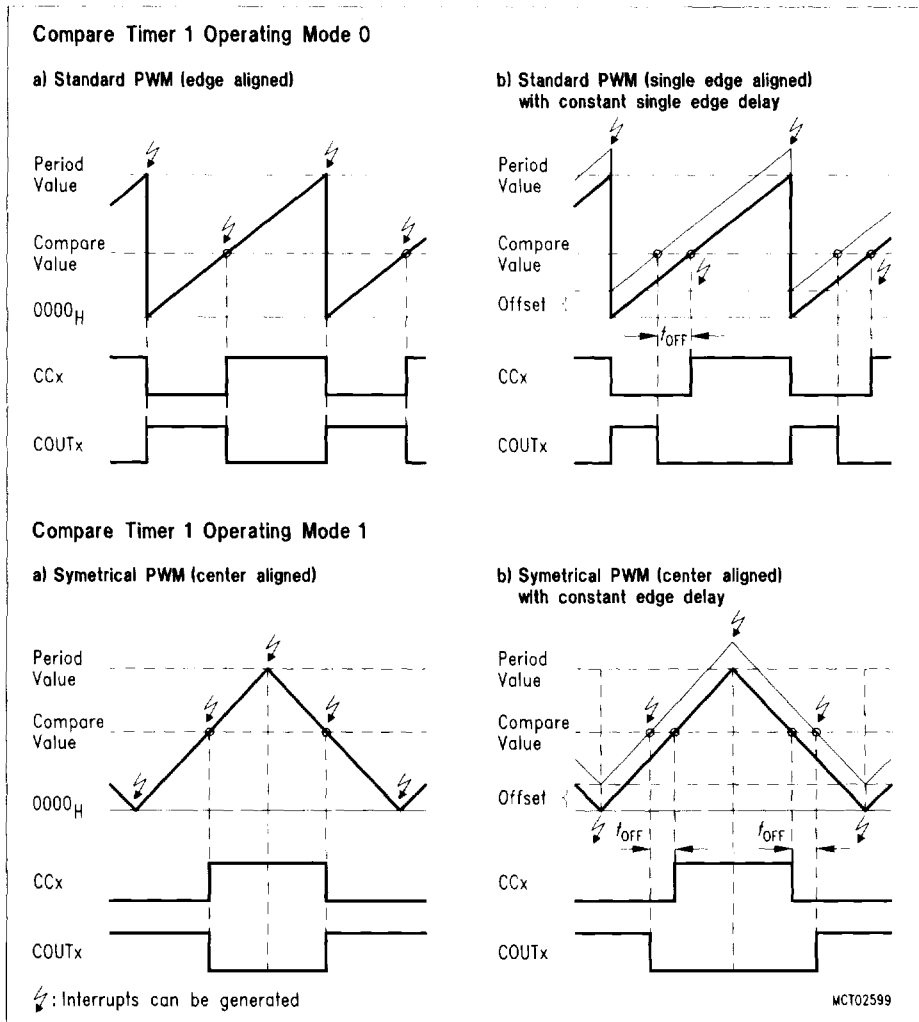
Figure 7 Basic Operating Modes of the CAPCOM Unit
