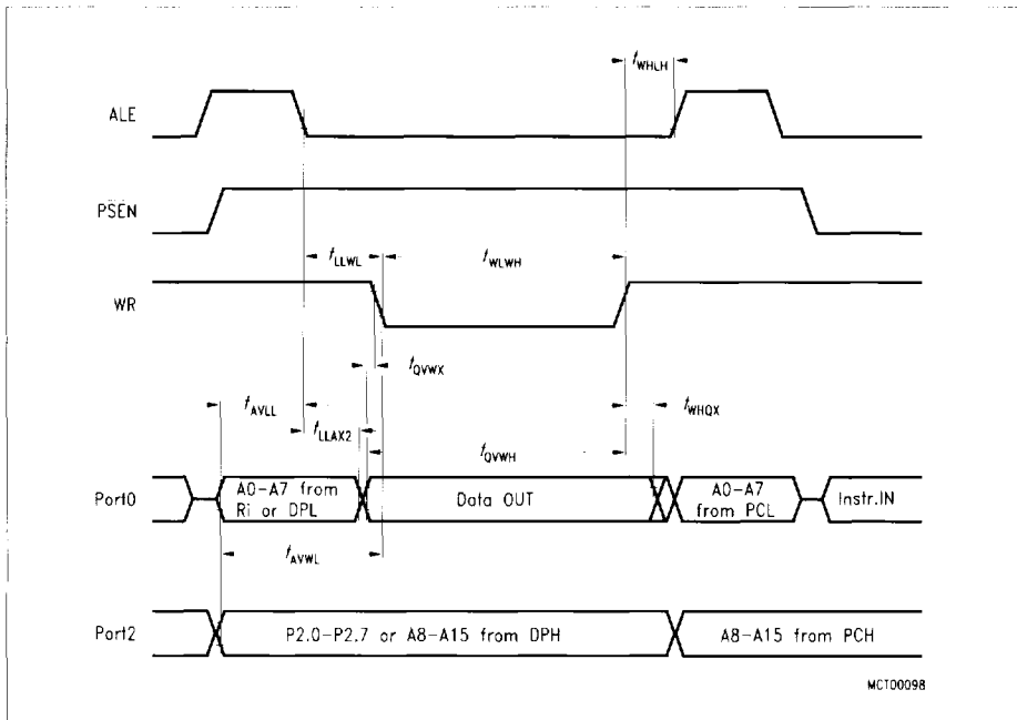
Figure 17 Data Memory Write Cycle
