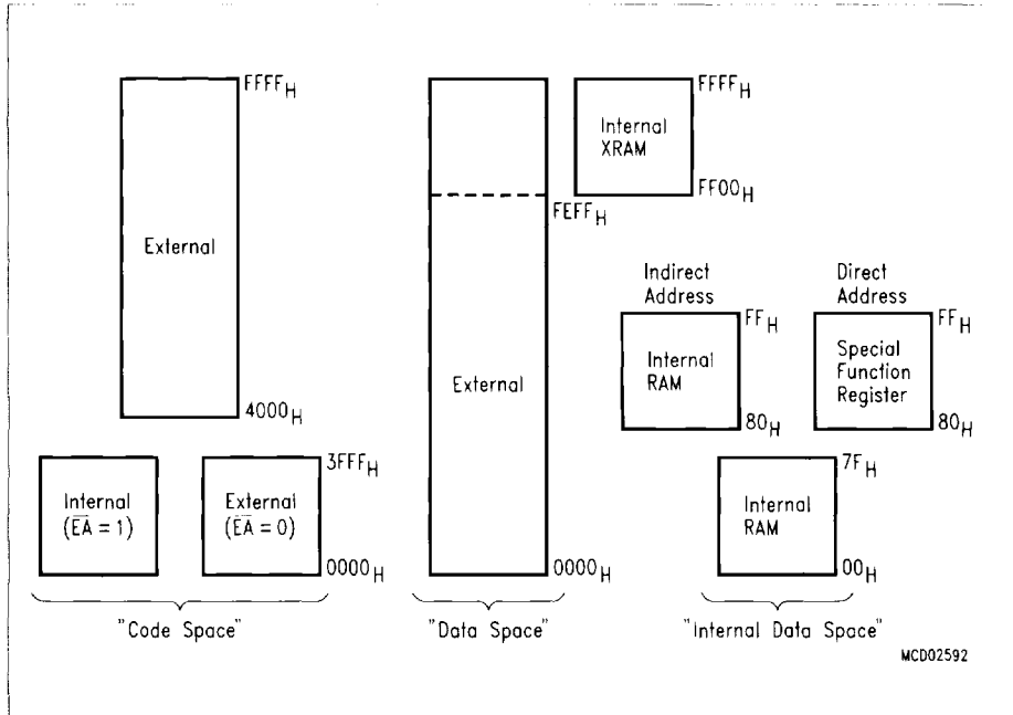
Figure 4 C504 Memory Map
