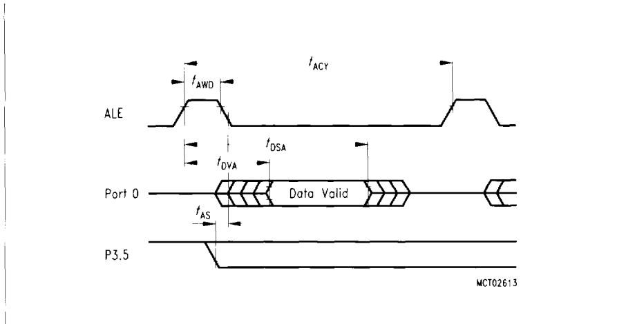
Figure 20 ROM Verification Mode 2
