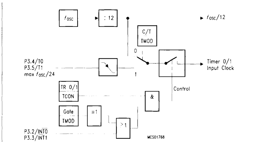
Figure 5 Timer/Counter 0 and 1 Input Clock Logic
