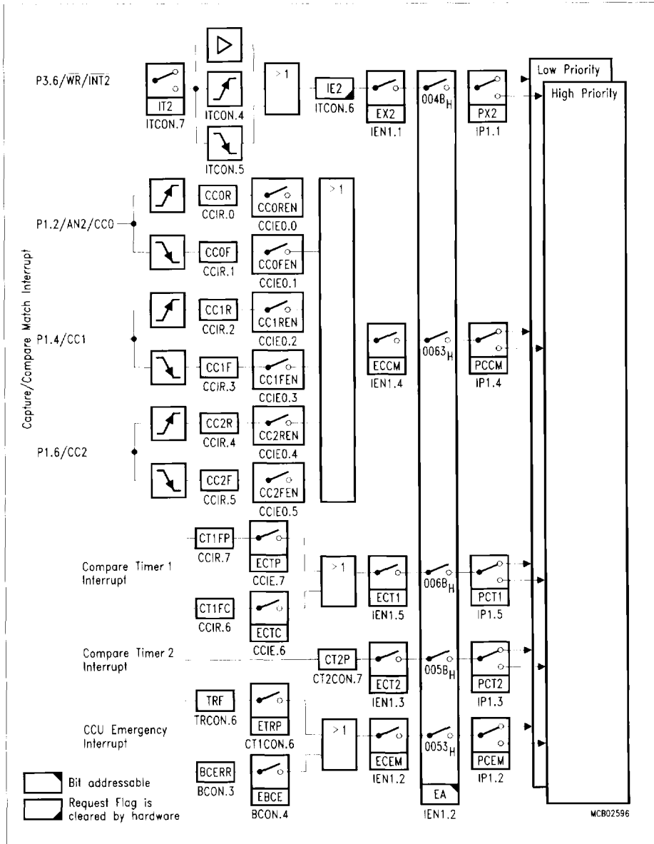
Figure 12 Interrupt Request Sources (Part 2)
