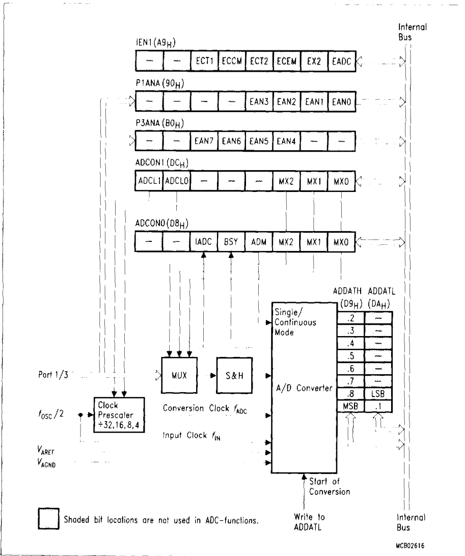
Figure 9 A/D Converter Block Diagram
