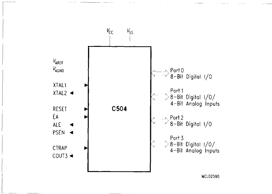
Figure 1 Logic Symbol
