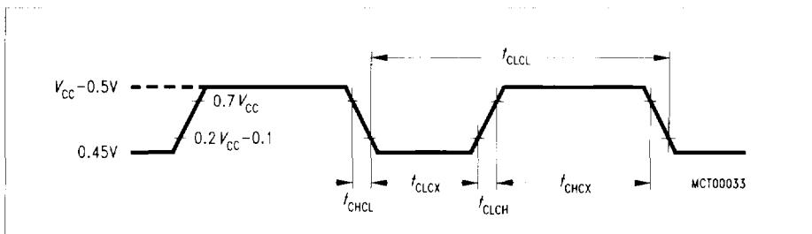
Figure 18 External Clock Cycle
