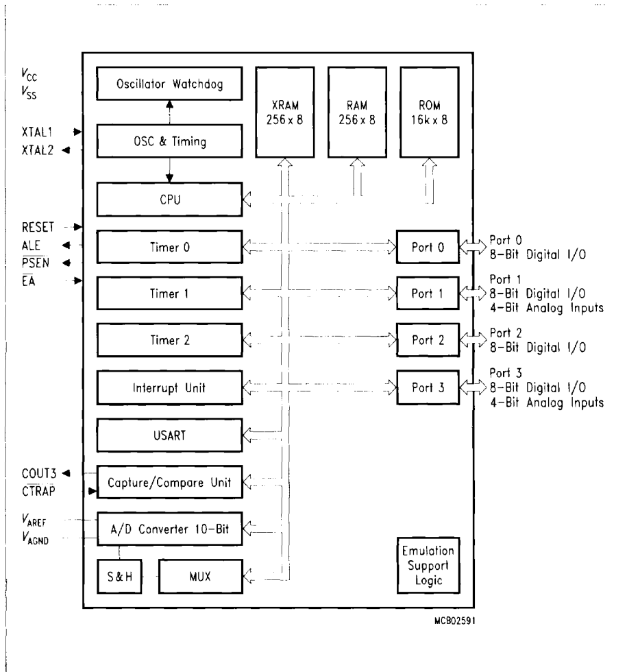
Figure 3 Block Diagram of the C504
