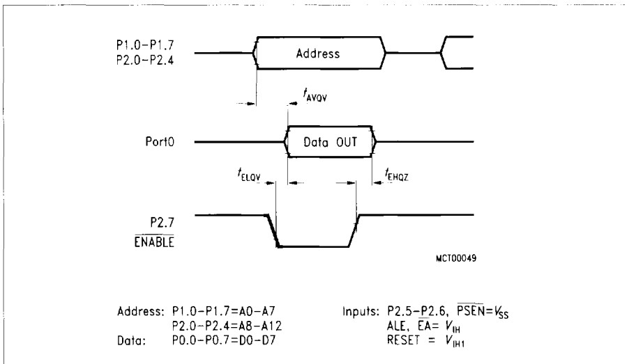
Figure 19 ROM Verification Mode 1
