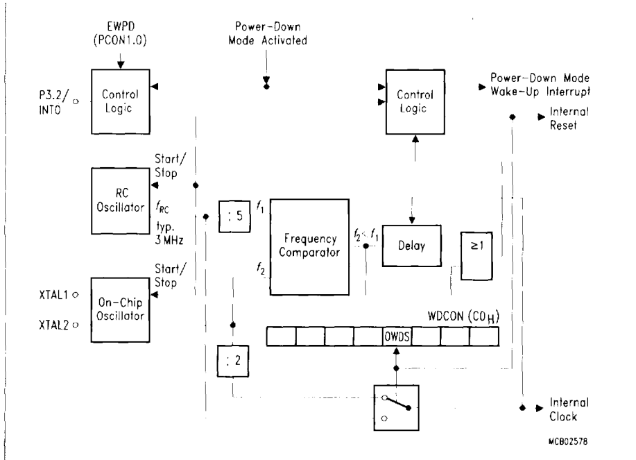
Figure 14 Block Diagram of the Programmable Watchdog Timer
