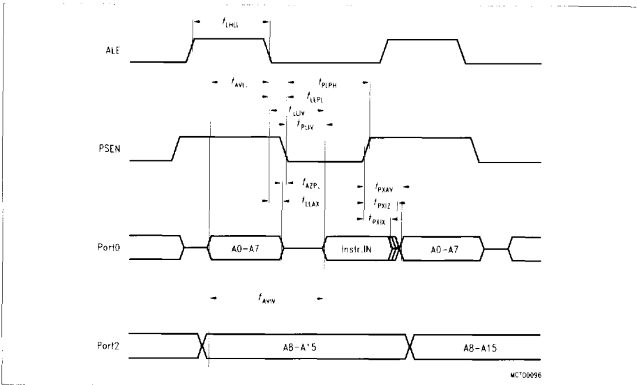
Figure 15 Program Memory Read Cycle
