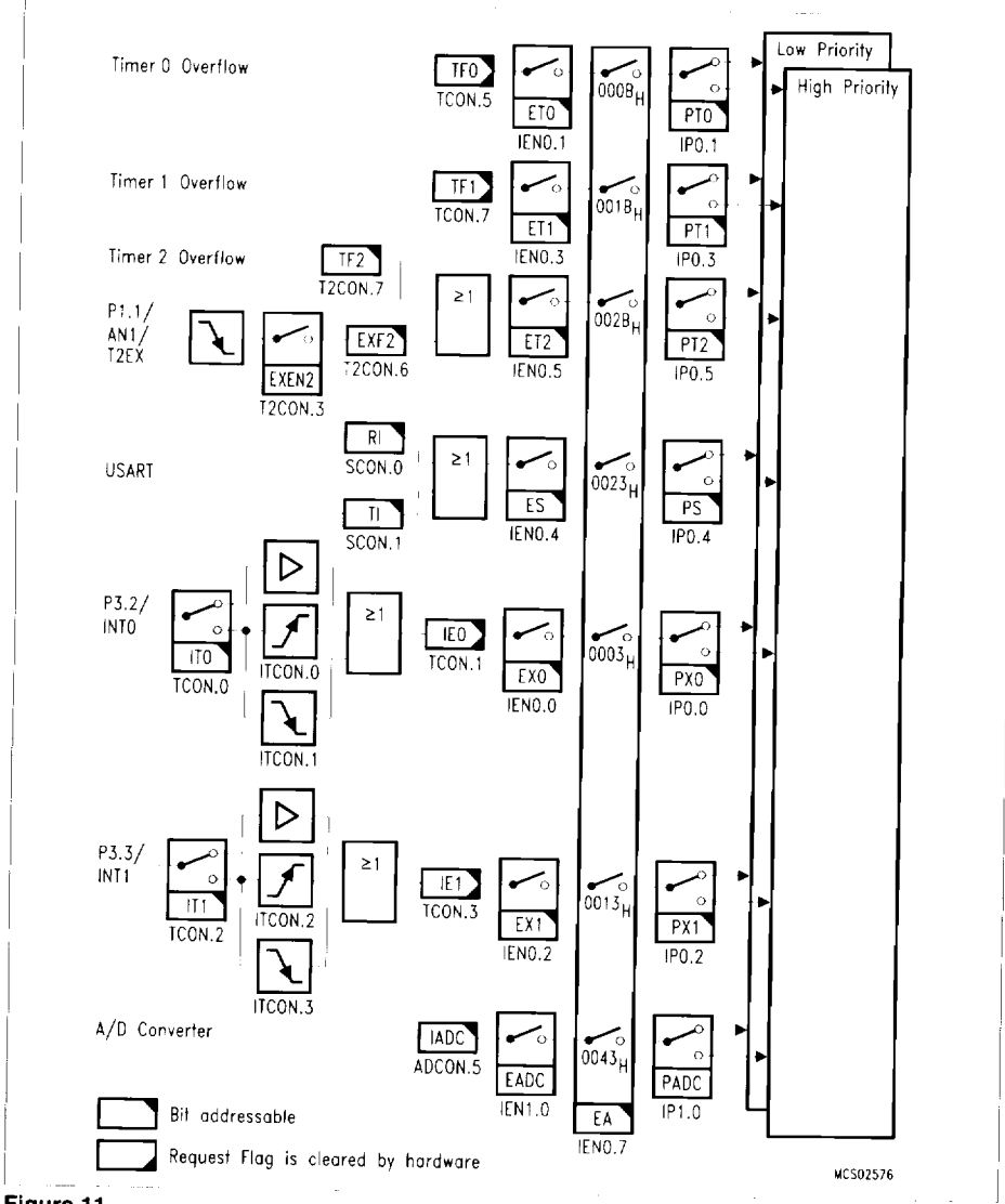
Figure 11 Interrupt Request Sources (Part 1)
