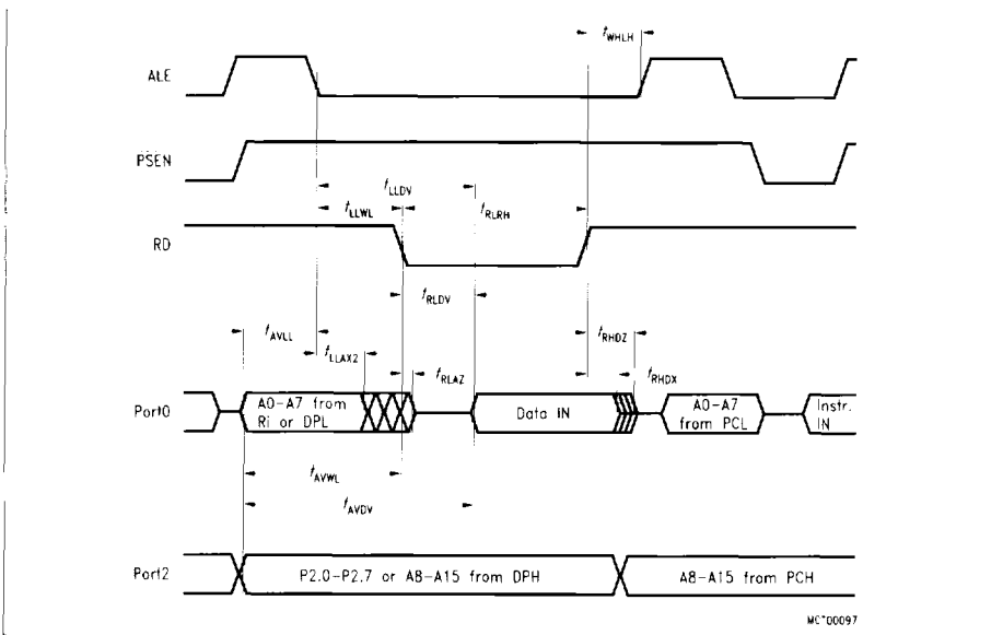
Figure 16 Data Memory Read Cycle
