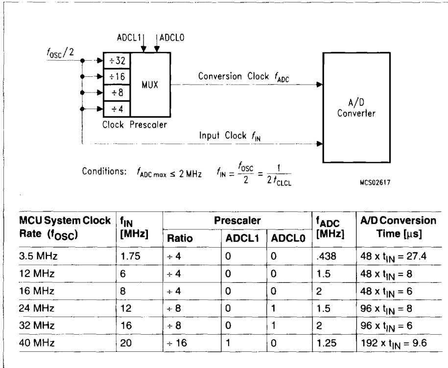
Figure 10 A/D Converter Clock Selection
