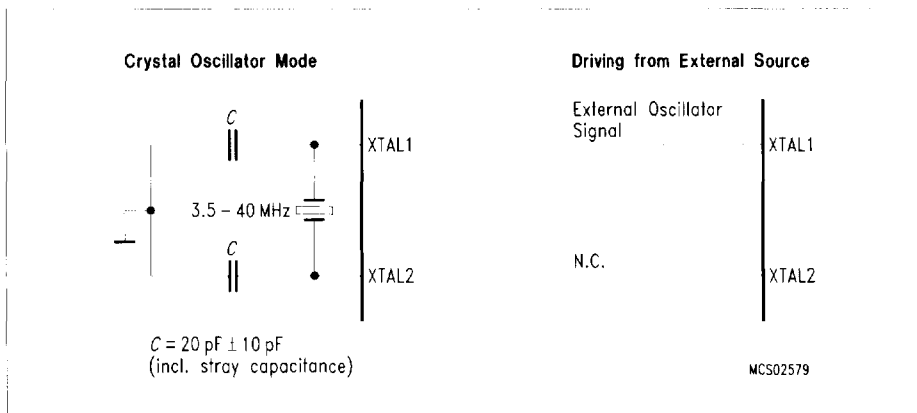
Figure 23 Recommended Oscillator Circuits for Crystal Oscillator
