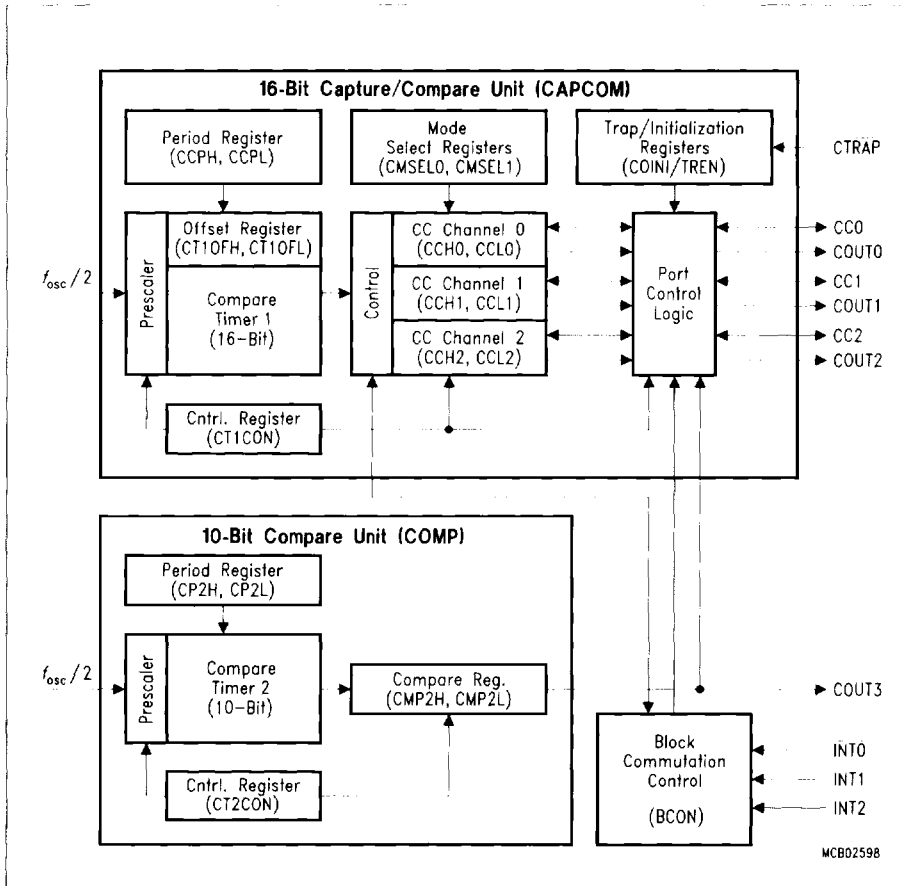
Figure 6 Block Diagram of the CCU
