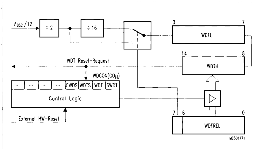
Figure 13 Block Diagram of the Programmable Watchdog Timer
