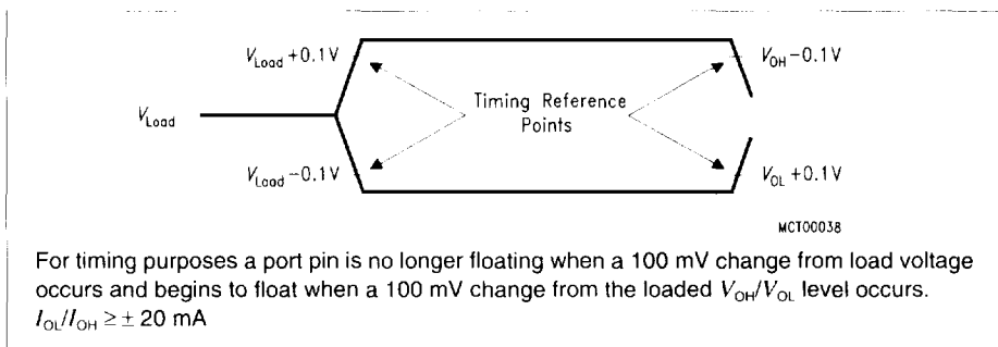
Figure 22 AC Testing : Float Waveforms
