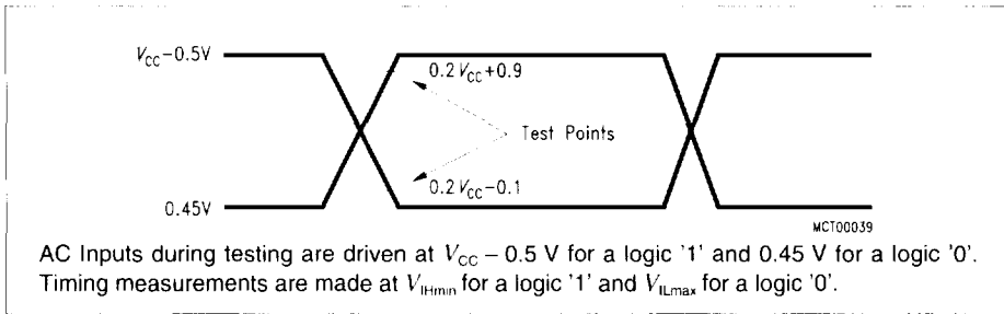
Figure 21 AC Testing: Input, Output Waveforms
