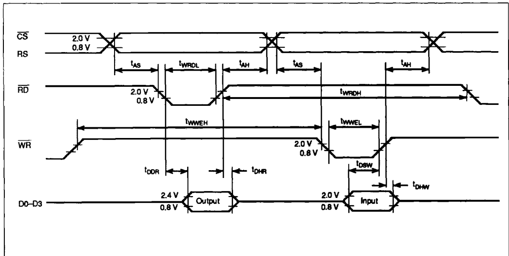
Figure 40 MPU Interface
