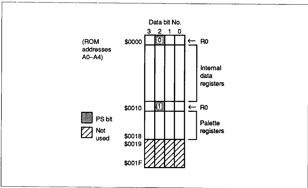
Figure 19 PS Bit Functions in ROM Programming Method
