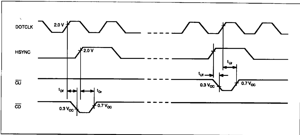
Figure 42 PLL Interface
