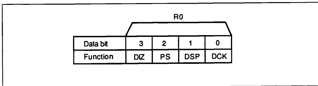
Figure 18 Control Register 1
