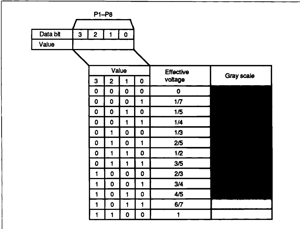
Figure 29 Palette Registers
