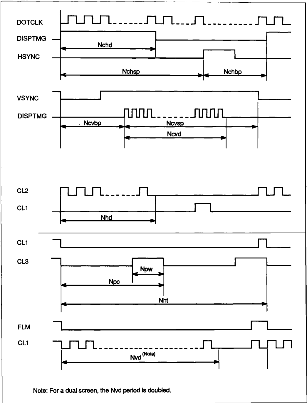
Figure 31 Symbol Definitions
