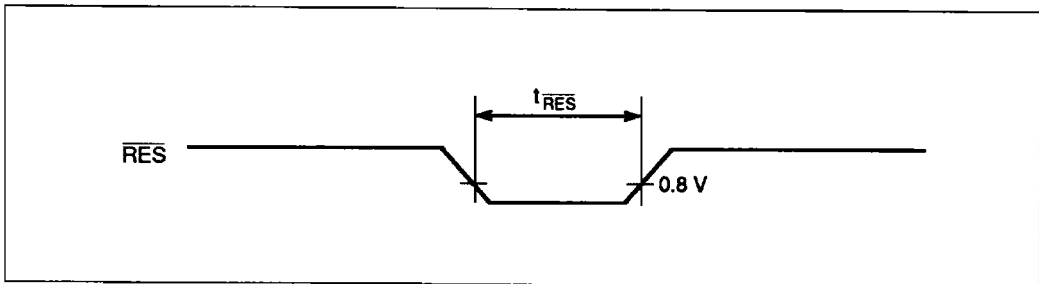
Figure 43 Reset Input
