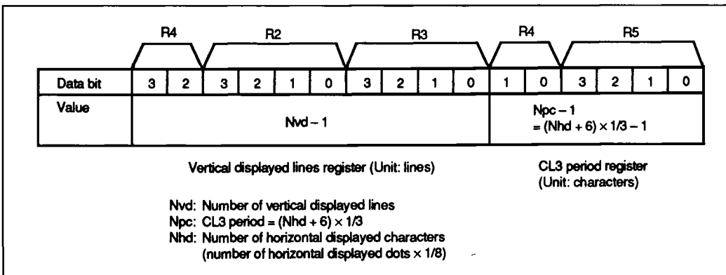
Figure 21 Vertical Displayed Lines Register and CL3 Period Register
