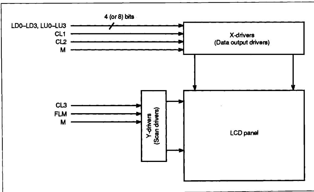
Figure 15 Connection for Double-Height Display
