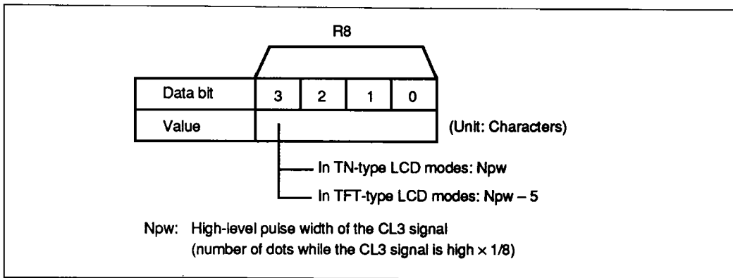
Figure 24 CL3 Pulse Width Register
