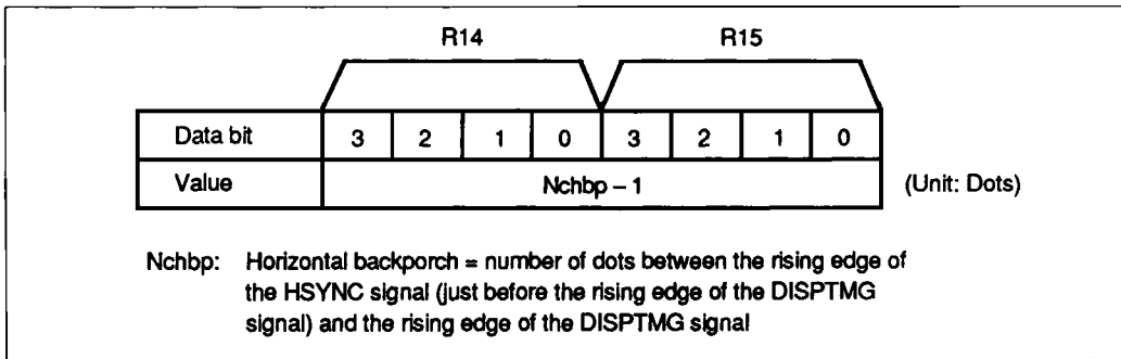
Figure 28 Horizontal Backporch Registers
