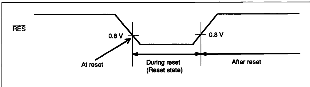
Figure 30 Reset Definition
