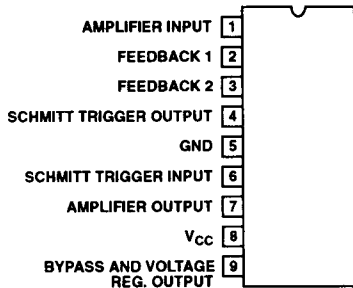
9-LEAD PLASTIC SIP TOP VIEW
