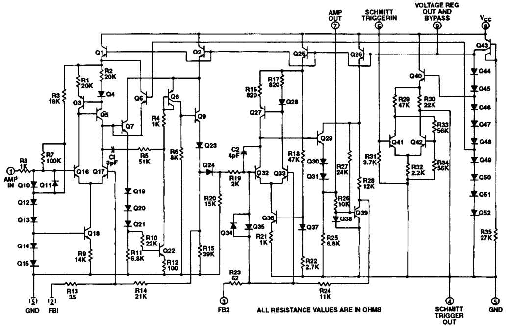
FIGURE 1. SCHEMATIC DIAGRAM FOR CA3237
