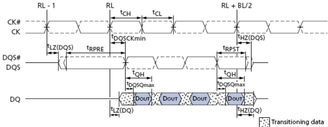
Data output (Read) timing ( t_{DQSCkmin} ), BL=4
