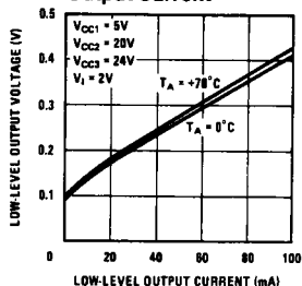
Low-Level Output Voltage vs Output Current
