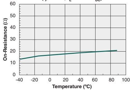
Typical On-Resistance vs. Temperature ( I_F=2\text{mA} , I_L=120\text{mA}_{\text{DC}} )
