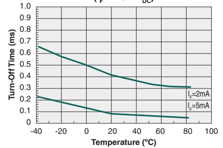
Typical Turn-Off Time vs. Temperature ( I_F=120\text{mA}_{\text{DC}} )
