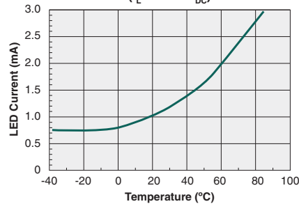
Typical I_F for Switch Dropout vs. Temperature ( I_L=120\text{mA}_{\text{DC}} )
