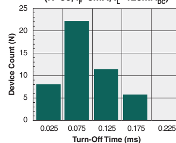
Typical Turn-Off Time (N=50, I_F=5\text{mA} , I_L=120\text{mA}_{DC} )
