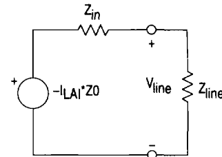
Figure 7. Replacement Diagram for the Transmit Amplifier
