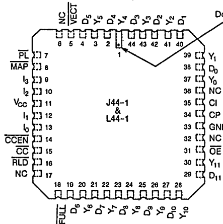
PLCC/LCC TOP VIEW
