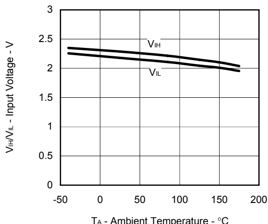
INPUT VOLTAGE vs. AMBIENT TEMPERATURE
