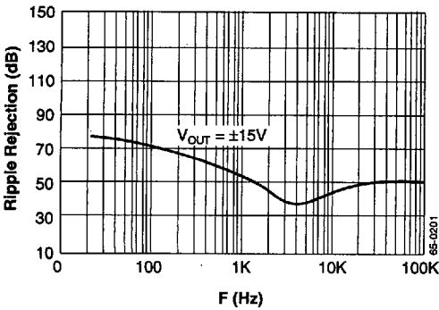
Figure 1. Ripple Rejection vs. Frequency
