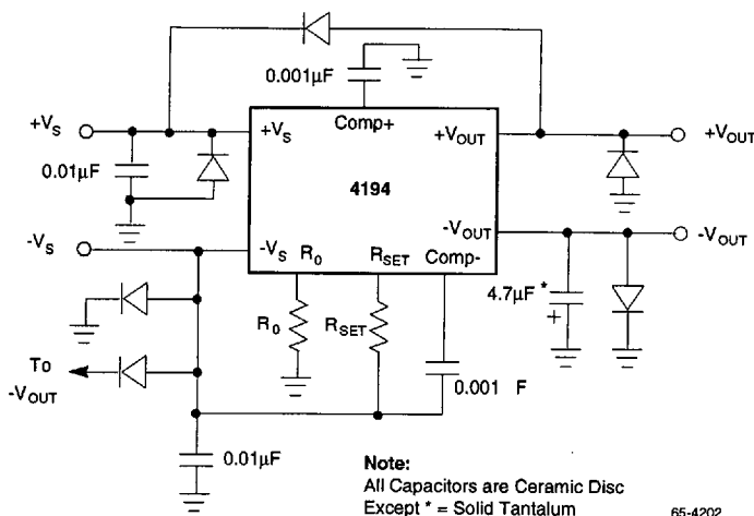
Figure 10. RC4194 Regulator Showing All Protective Diodes
