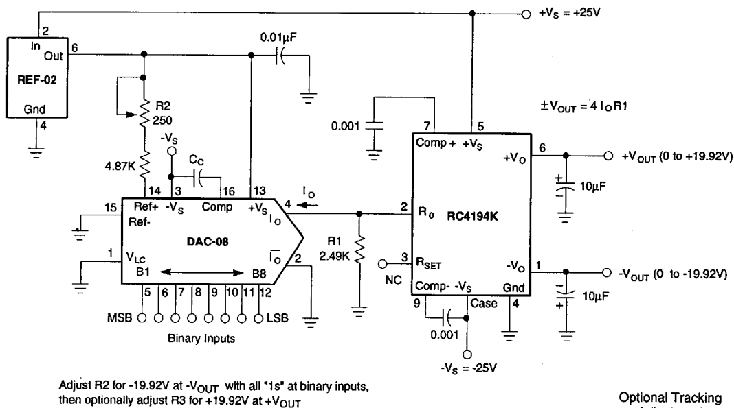
Figure 6. Balanced Output Voltage — Op Amp Application
