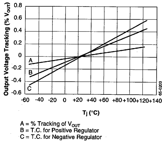
Figure 3. Output Voltage Tracking vs. Temperature
